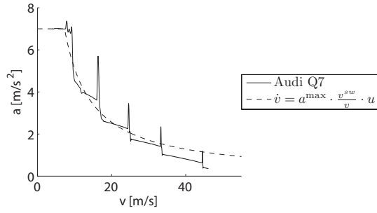
Fig. 5. Maximum acceleration a of the Audi Q7 plotted over its velocity v ; used parameters: a^{\max} = 7 \text{ [m/s}^2\text{]} , v^{\text{sw}} = 7.3 \text{ [m/s]} .
