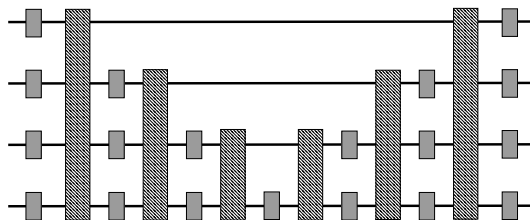
Fig. 1. In quantum optics, passive transformations on n modes are in one-to-one correspondence with n \times n unitaries. Up to an overall phase, each unitary U admits a decomposition into 2(n-1) canonical multiports (which are independent of U and described by discrete Fourier transformations [hatched]) surrounded by 2n-1 layers of single-mode phase shifters [grey]. Here, this is exemplified for n=4 .
