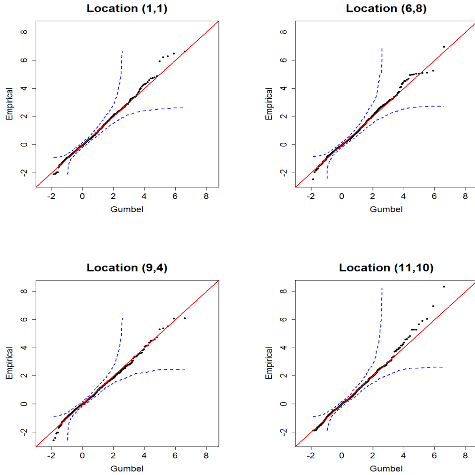
Figure 5.2: qq-plots of the Gumbel transformed time series values versus the standard Gumbel distribution for four locations: (1,1) (top left), (6,8) (top right), (9,4) (bottom left) and (11,10) (bottom right). Dashed blue lines mark 95% confidence bounds. Solid red lines correspond to no deviation.
