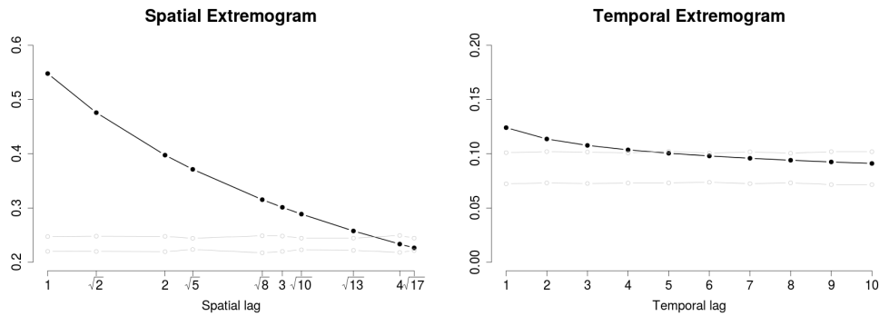
Figure 3.6: Permutation test for extremal independence: The gray lines show the 97.5%— and 2.5%—quantiles of the extremogram estimates for 1000 random space-time permutations for the empirical spatial (left) and the temporal (right) extremogram estimates.
