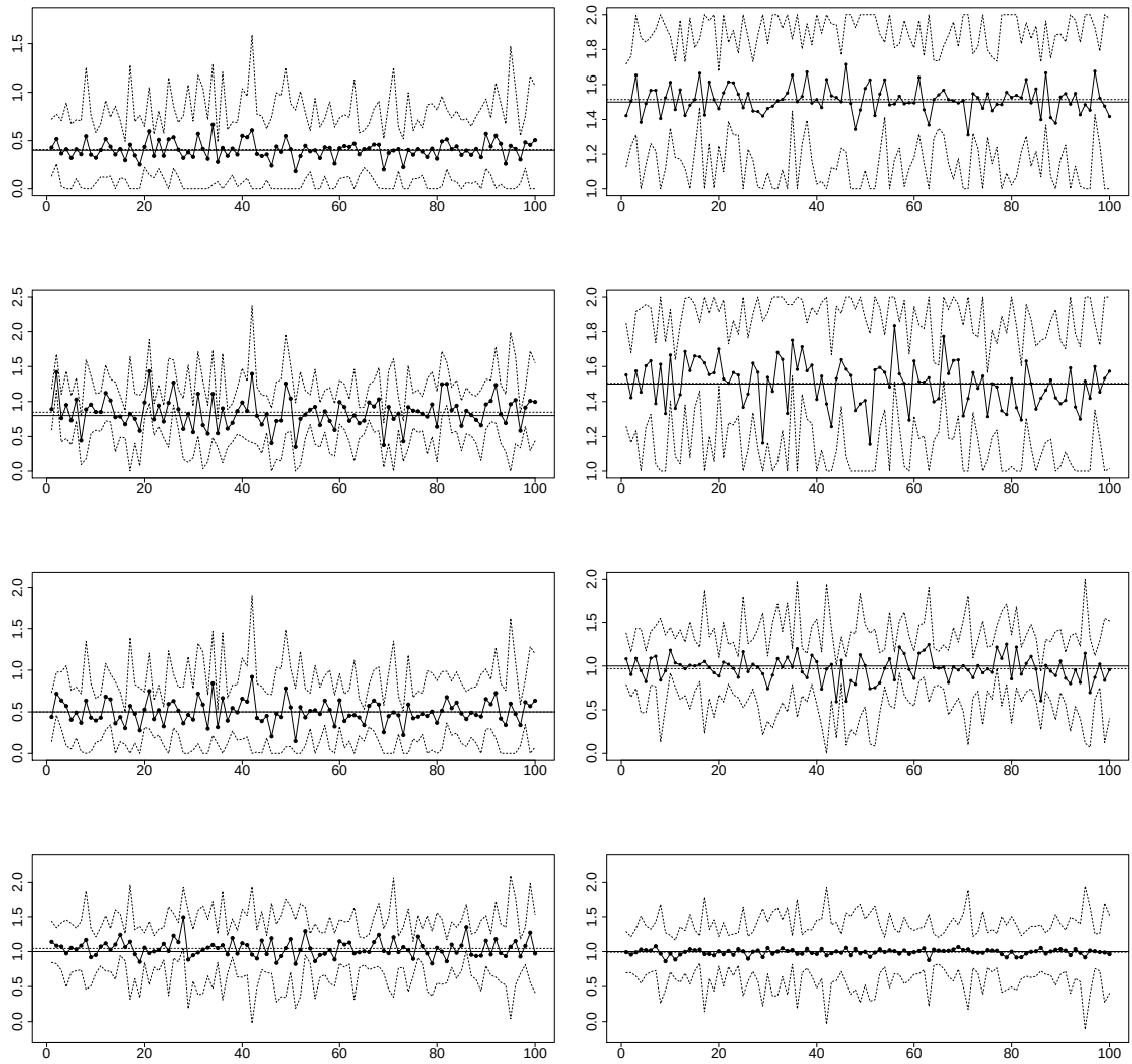
Figure 4.3: GLSEs of the parameters of model (iii) for 100 simulated Brown-Resnick space-time processes together with pointwise 95%-subsampling confidence intervals (dotted). First row: C_1, \alpha_1 , second row: C_2, \alpha_2 , third row: C_3, \alpha_3 , fourth row: \tau_1, \tau_2 . The middle solid line is the true value and the middle dotted line represents the mean over all estimates.
