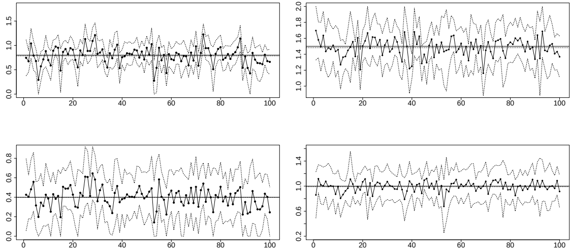
Figure 4.1: GLSEs of the parameters of model (i) for 100 simulated Brown-Resnick space-time processes together with pointwise 95%-subsampling confidence intervals (dotted). First row: C_1 , \alpha_1 , second row: C_2 , \alpha_2 . The middle solid line is the true parameter value and the middle dotted line represents the mean over all estimates.
