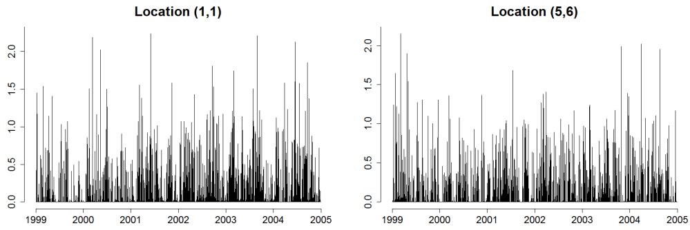
Figure 3.4: Daily rainfall maxima over hourly accumulated measurements from 1999-2004 in inches for two grid locations.
