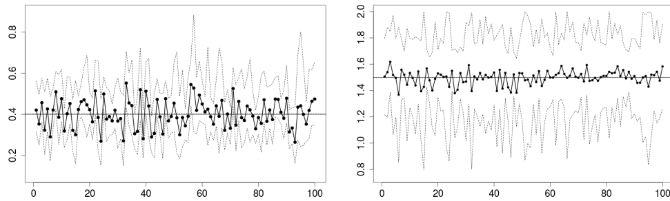
Figure 3.2: WLSEs of \theta_1 (left) and \alpha_1 (right) for 100 simulated Brown-Resnick space-time processes together with pointwise 95%–subsampling confidence intervals (dotted). The middle solid line is the true value and the middle dotted line represents the mean over all estimates.
