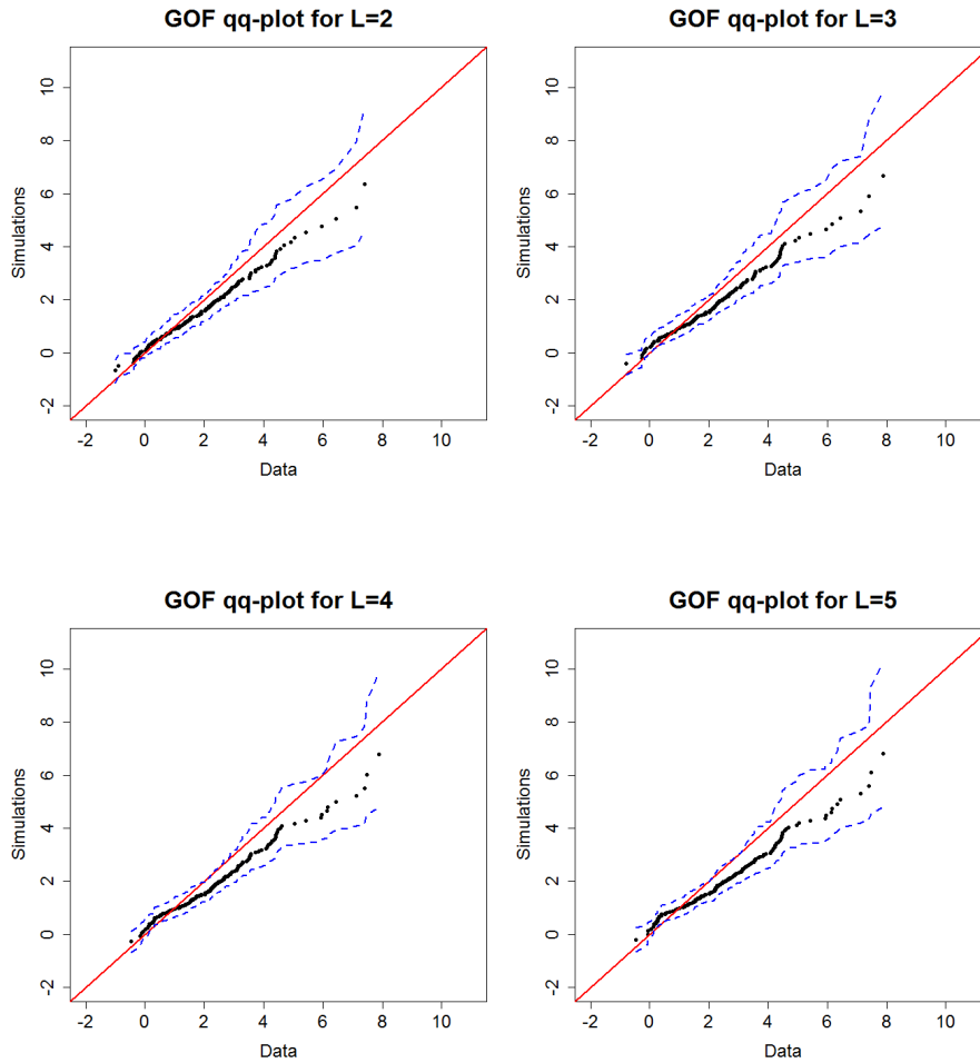
Figure 5.5: Goodness of fit qq-plots for different spatial locations and different L . Top left: L = 2 : (1,1) and (1,2). Top right: L = 3 : (1,1), (1,2) and (3,1). Bottom left: L = 4 : (1,1), (1,2), (3,1) and (3,2). Bottom right: L = 5 : (1,1), (1,2), (3,1), (3,2) and (2,1). PMLEs underlying the simulations are based on maximum spatial and temporal lags 4 and 2, respectively. Dashed blue lines mark 95% pointwise confidence bounds. Solid red lines correspond to no deviation.
