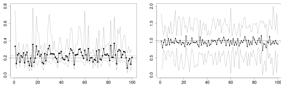
Figure 3.3: WLSEs of \theta_2 (left) and \alpha_2 (right) for 100 simulated Brown-Resnick space-time processes together with pointwise 95%–subsampling confidence intervals (dotted). The middle solid line is the true value and the middle dotted line represents the mean over all estimates.
