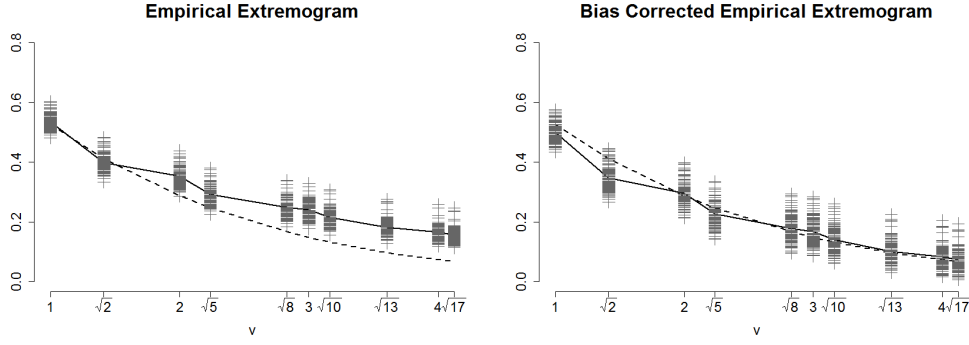
Figure 3.1: Empirical spatial extremogram (left) and its bias corrected version (right) for one hundred simulated max-stable random fields in (3.1) with \delta(v, 0) = 2 \cdot 0.4v^{1.5} . The dotted line represents the theoretical spatial extremogram and the solid line is the mean over all estimates.
