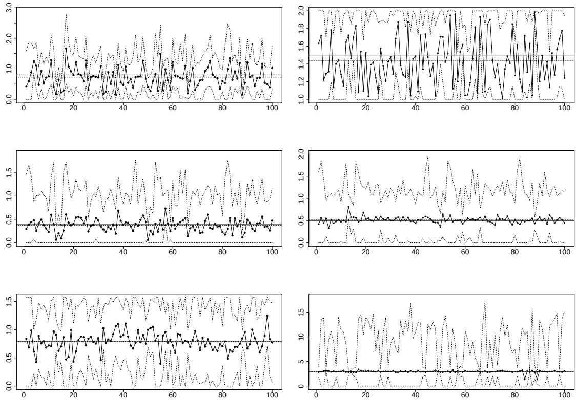
Figure 4.2: GLSEs of the parameters of model (ii) for 100 simulated Brown-Resnick space-time processes together with pointwise 95%-subsampling confidence intervals (dotted). First row: C_1 , \alpha_1 , middle row: C_2 , \alpha_2 , last row: \varphi and c . The middle solid line is the true value and the middle dotted line represents the mean over all estimates.
