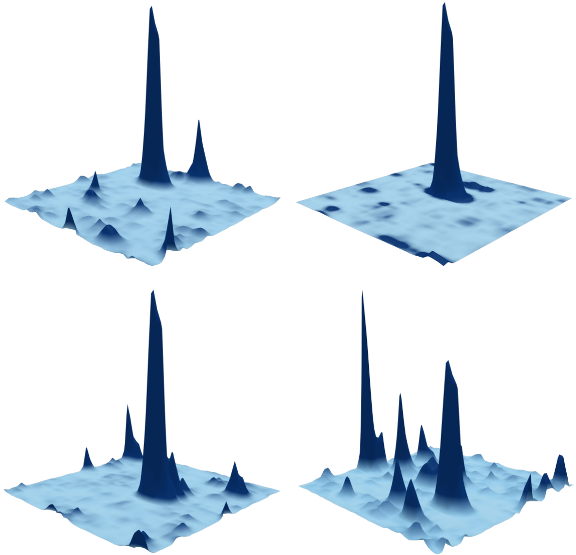
Figure 1.4: Simulation from a time-shifted Brown-Resnick space-time model shown at four consecutive time points (from left to right and top to bottom). The movement and scaling of the largest peak in the top left plot from the upper corner of the grid to the lower corner in the bottom right plot is clearly visible. Also smaller peaks can be observed to emerge and disappear.
