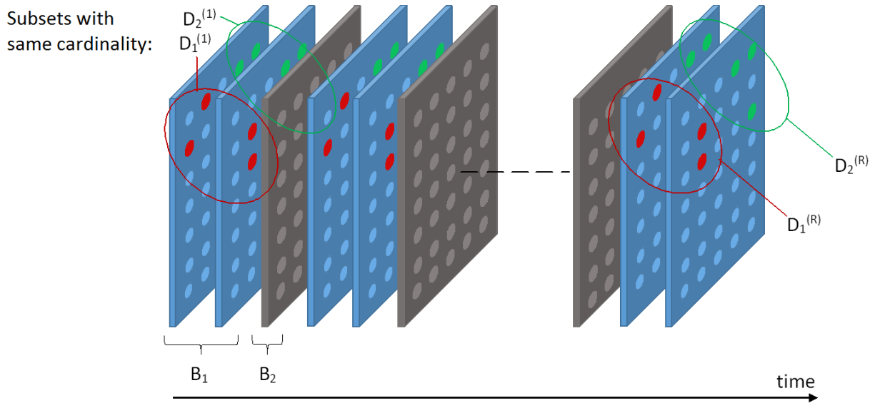
Figure 5.3: R independent realisations of \eta_D for different subsets D of the space-time observation area.
