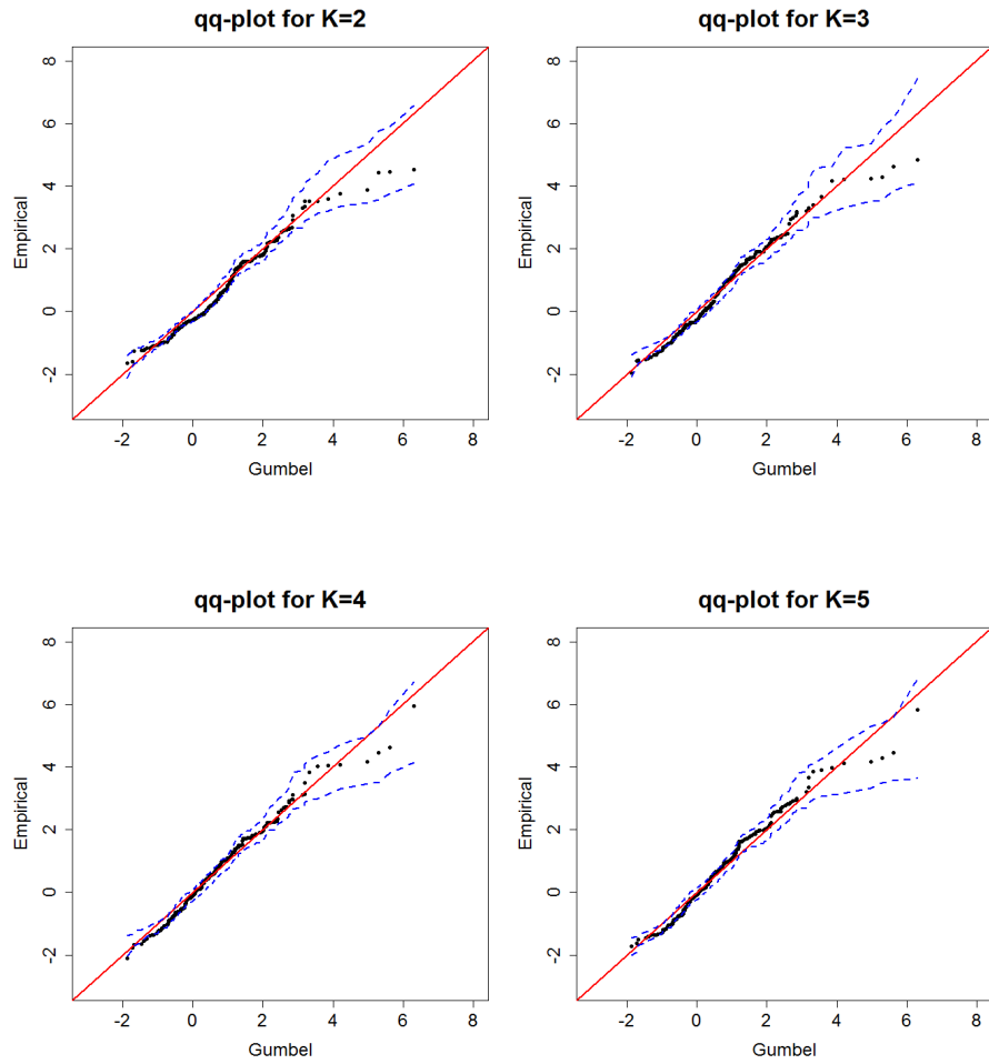
Figure 5.4: qq-plots of theoretical standard Gumbel quantiles versus the empirical quantiles (black dots). The latter correspond to the empirical distribution of maxima taken over groups of cardinality K . Dashed blue lines mark 95% pointwise confidence bounds obtained by block bootstrap. Solid red lines correspond to no deviation.
