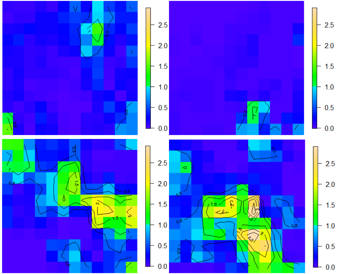
Figure 1.3: Daily rainfall maxima in inches taken over hourly accumulated measurements at 144 gridded locations in Florida, USA, and at four consecutive days (from left to right and top to bottom) in the period 1999-2004.
