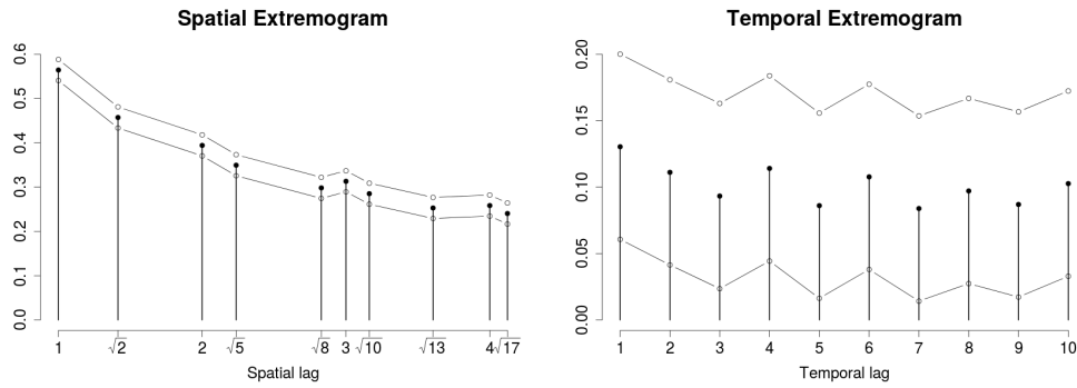
Figure 3.5: Empirical spatial (left) and temporal (right) extremogram based on spatial and temporal means for the space-time observations as given in (3.10) and (3.11) together with 95%—subsampling confidence intervals.
