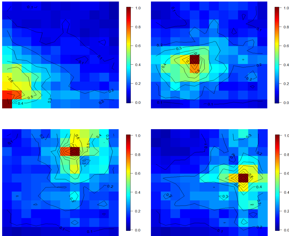
Figure 5.6: Predicted conditional probability fields based on daily maxima for reference space-time points (1,1,1) , (5,6,1) , (8,10,1) and (10,7,1) and rainfall levels z = z^* = 2.5 (clockwise from the top left to the bottom right).
