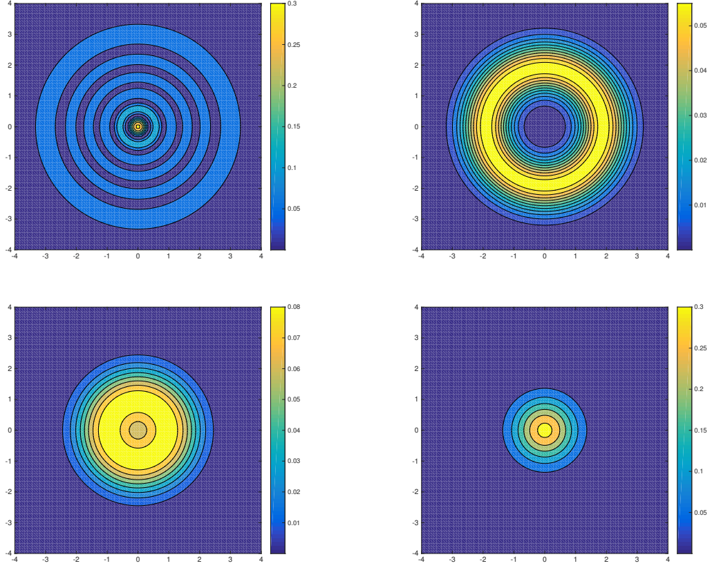
Figure 17.: Contour plots of the absolute values of \mathcal{U}(t)\mathcal{W}_{(5,5)}(\mathcal{Z}) at time t = 0 (upper left), t = 0.5 (upper right), t = 1 (lower left) and t = 4 (lower right) for \varepsilon = 1
