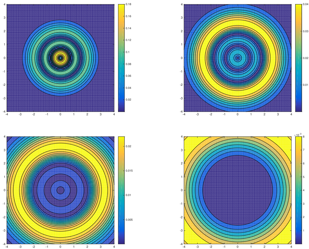
Figure 21.: Contour plots of the absolute values of \widehat{\mathcal{U}}(t)\mathcal{W}_{(3,2)}(\mathcal{Z}) at time t = 0 (upper left), t = 0.2 (upper right), t = 0.4 (lower left) and t = 0.08 (lower right) for \alpha = 1 , \beta = i and \varepsilon = 1
