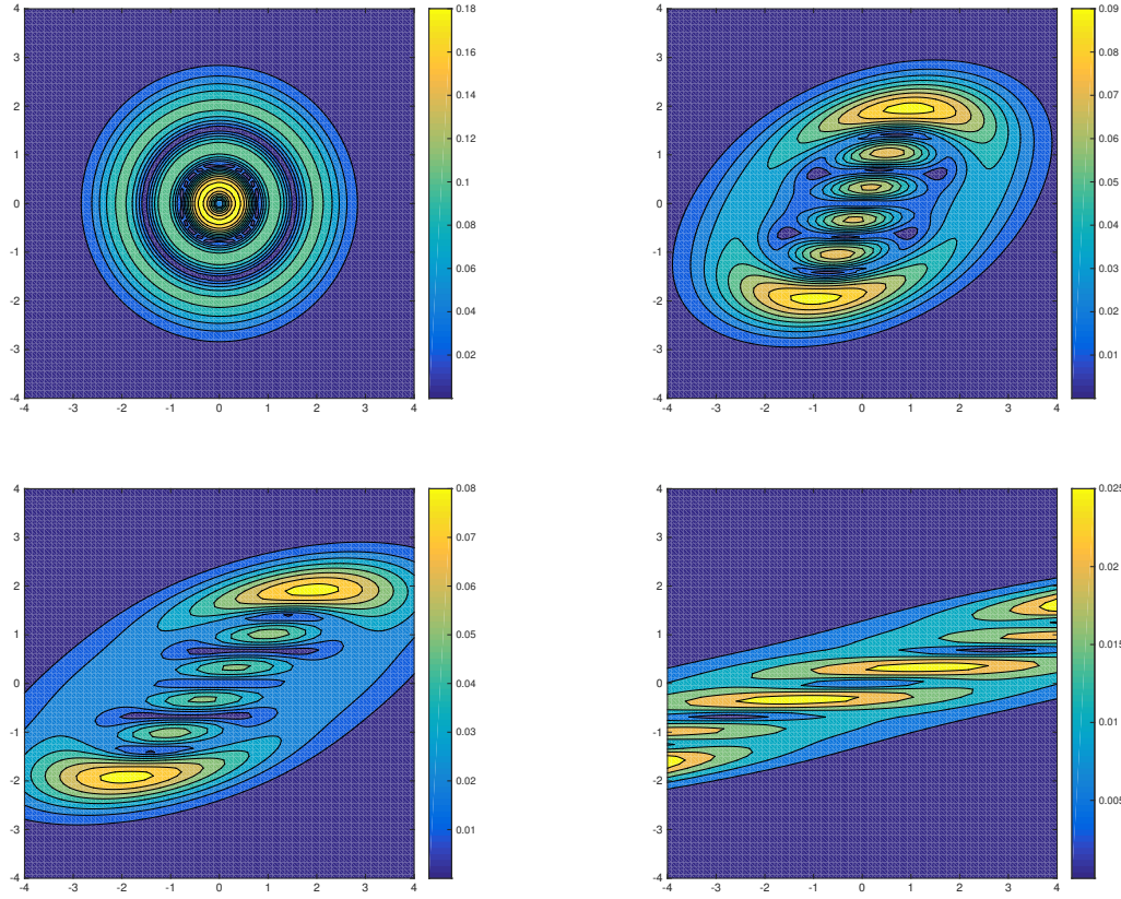
Figure 24.: Contour plots of the absolute values of \hat{\mathcal{U}}(t)\mathcal{W}_{(3,2)}(\mathcal{Z}) at time t = 0 (upper left), t = 0.5 (upper right), t = 1 (lower left) and t = 4 (lower right)
