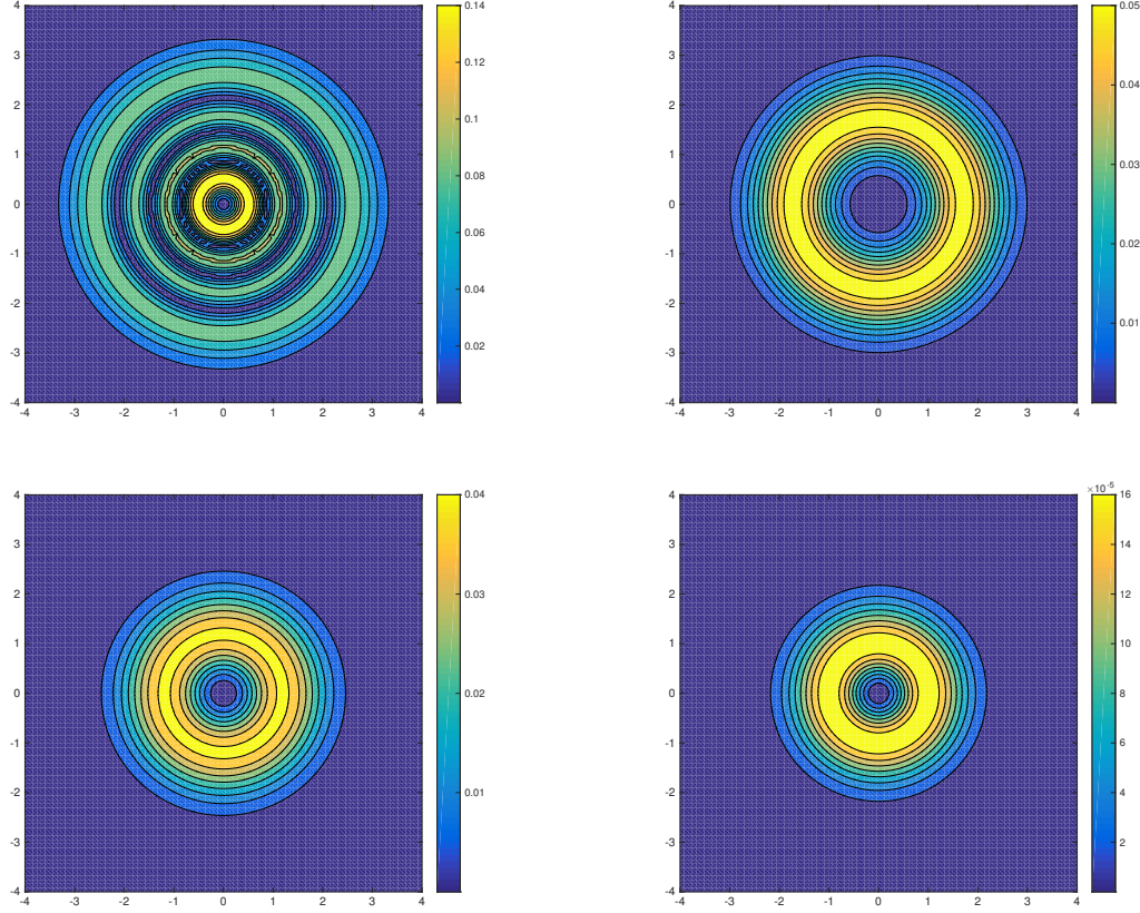
Figure 18.: Contour plots of the absolute values of \widehat{\mathcal{U}}(t)\mathcal{W}_{(5,3)}(\mathcal{Z}) at time t = 0 (upper left), t = 0.5 (upper right), t = 1 (lower left) and t = 4 (lower right) for \varepsilon = 1
