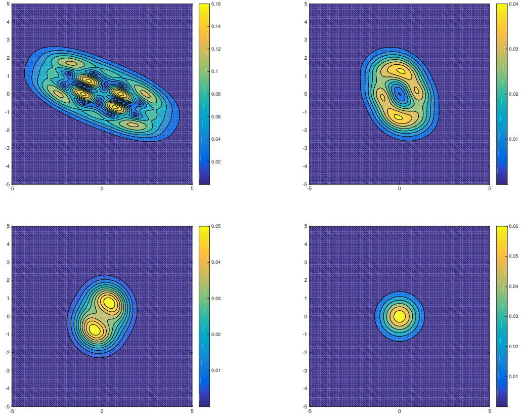
Figure 19.: Contour plots of the absolute values of \widehat{U}(t)\mathcal{W}_{(2,2)}(\mathcal{Z}) at time t = 0 (upper left), t = 0.5 (upper right), t = 1 (lower left) and t = 4 (lower right) for \varepsilon = 1
