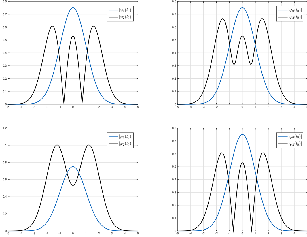
Figure 13.: Absolute values of the wave packets \varphi_0(l_t) and \varphi_2(l_t) starting from l_0 = (i, 1)^T at time t = 0 (upper left), t = 0.3925 \approx \frac{\pi}{8} (upper right), t = 1.57 \approx \frac{\pi}{2} (lower left) and t = 3.14 \approx \pi (lower right) for \varepsilon = 1 and \omega_0 = 1 .
