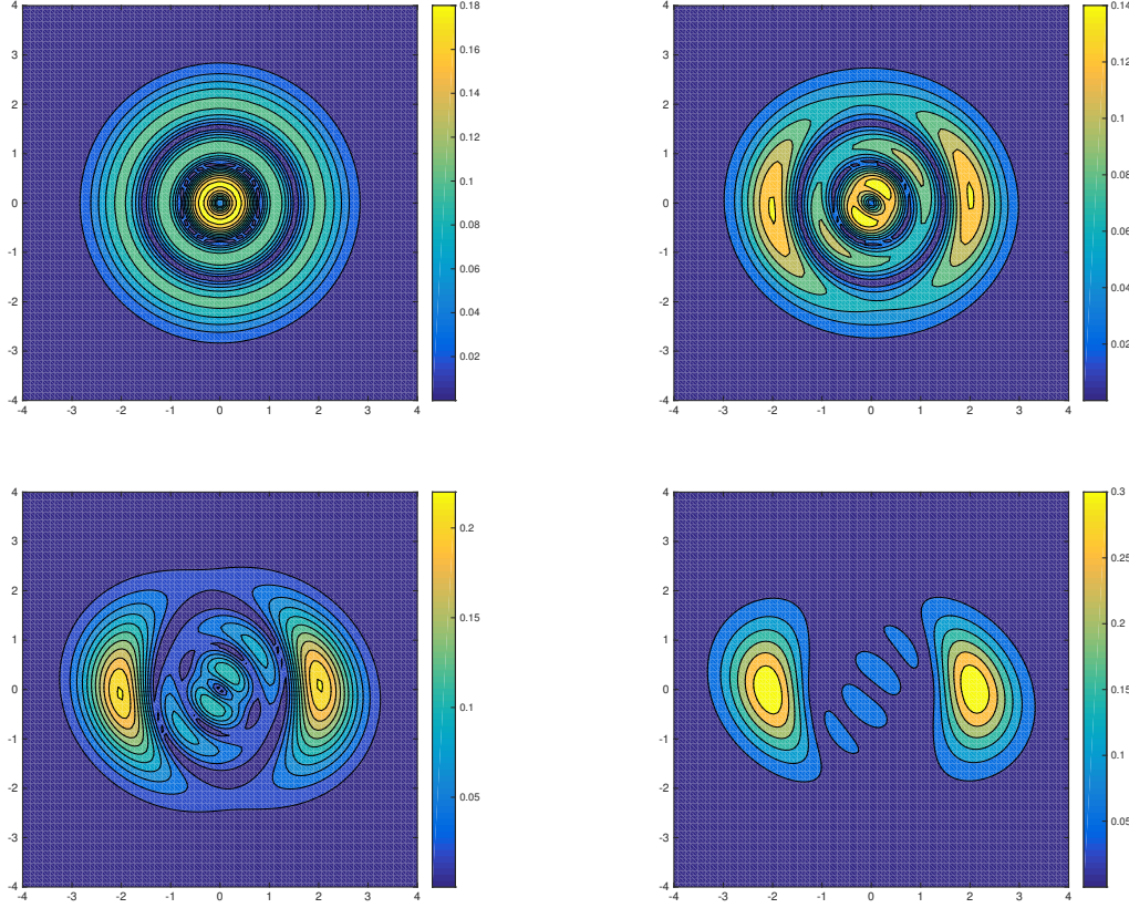
Figure 20.: Contour plots of the absolute values of \hat{\mathcal{U}}(t)\mathcal{W}_{(3,2)}(\mathcal{Z}) at time t = 0 (upper left), t = 0.01 (upper right), t = 0.03 (lower left) and t = 0.06 (lower right) for \alpha = 1, \beta = 2 and \varepsilon = 1
