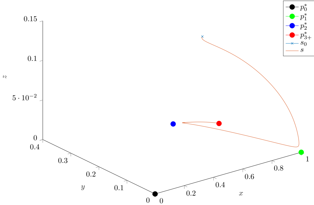
Figure 2.5.11: For b = 0.7 the solution converges to the asymptotically stable equilibrium p_{3+}^* as t \rightarrow \infty
