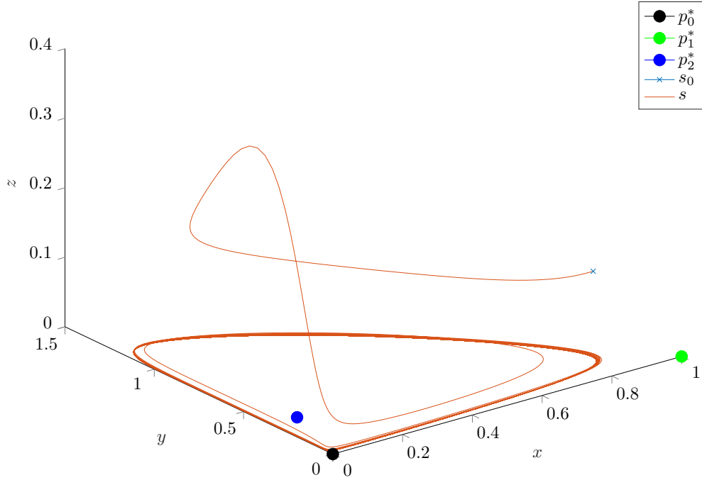
Figure 2.5.7: For b = 0.2 the positive phase curve approaches the periodic orbit \Gamma_{per}^* as t \rightarrow \infty
