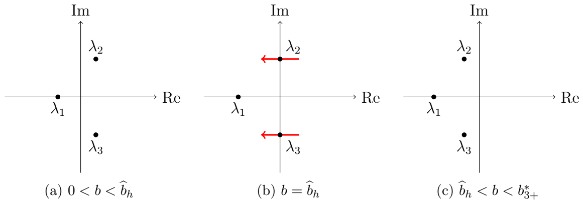
Figure 2.4.21: The eigenvalues \lambda_{2/3} cross the imaginary axis for b = \hat{b}_h \in (0, b_{3+}^*) .
