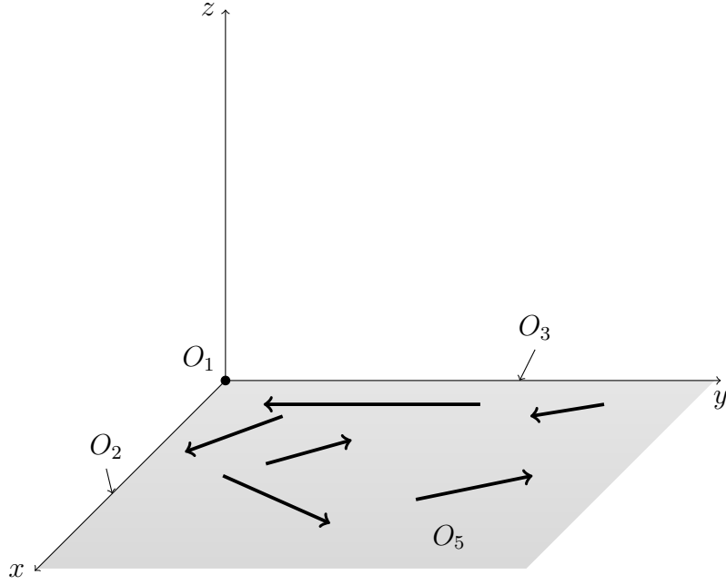
Figure 2.1.3: Schematic figure of a vector field tangent to the set O_5 \subset \mathcal{O}_0^+ .
