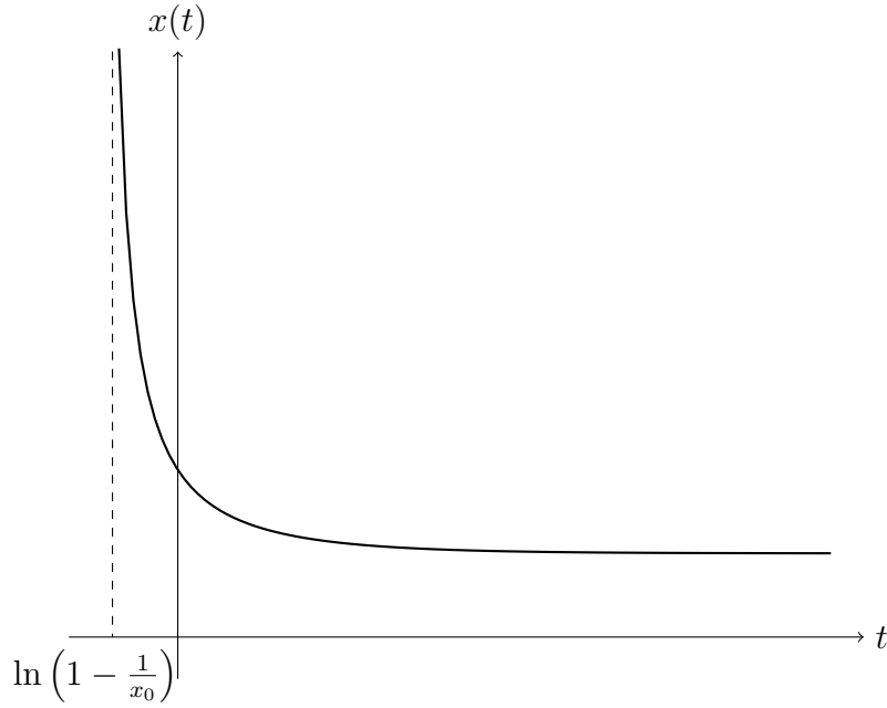
Figure 2.1.4: For the initial condition s_0 = (x_0, 0, 0) and x_0 > 1 the first component of the solution s diverges as t \rightarrow \ln\left(1 - \frac{1}{x_0}\right) .
