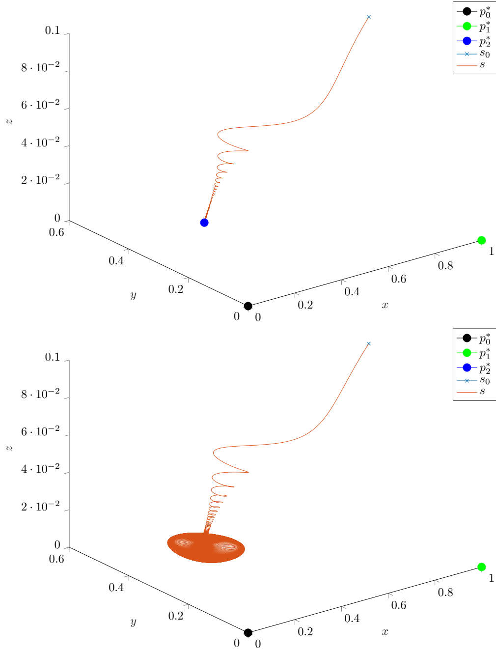
Figure 2.5.4: The cases b = 0.54 (top) and b = 0.53 (bottom), close to the Hopf bifurcation value b = \frac{7}{13} \approx 0.5385
