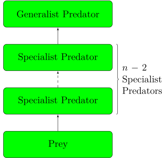
Figure 3.2.1: Scheme of the canonical n -dimensional GSP food chain, see (3.2.1)
