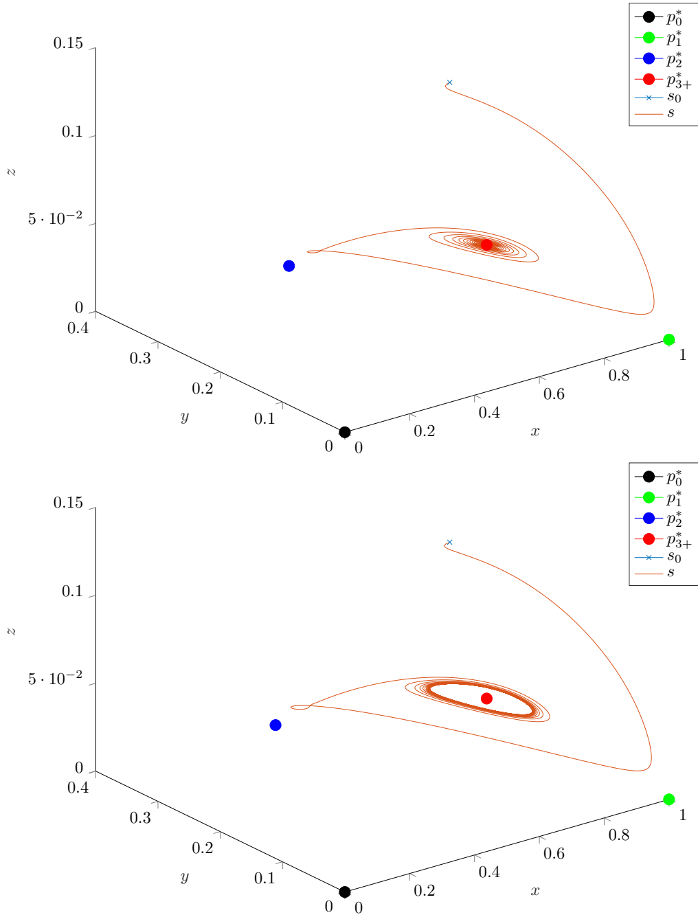
Figure 2.5.12: The cases b = 0.65 (top) and b = 0.64 (bottom), close to the Hopf bifurcation value \hat{b} \approx 0.6451
