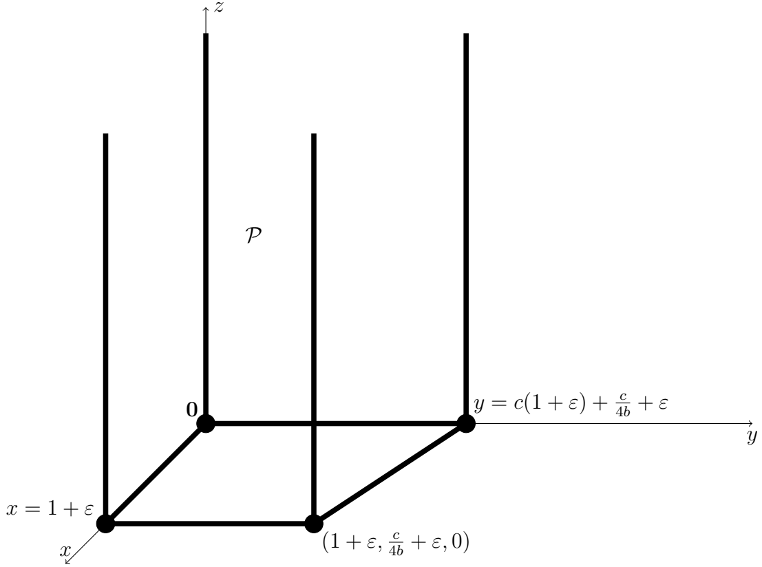
Figure 2.3.3: The set \mathcal{P} \subset \mathcal{O}_0^+ is a semi-infinite prism.
