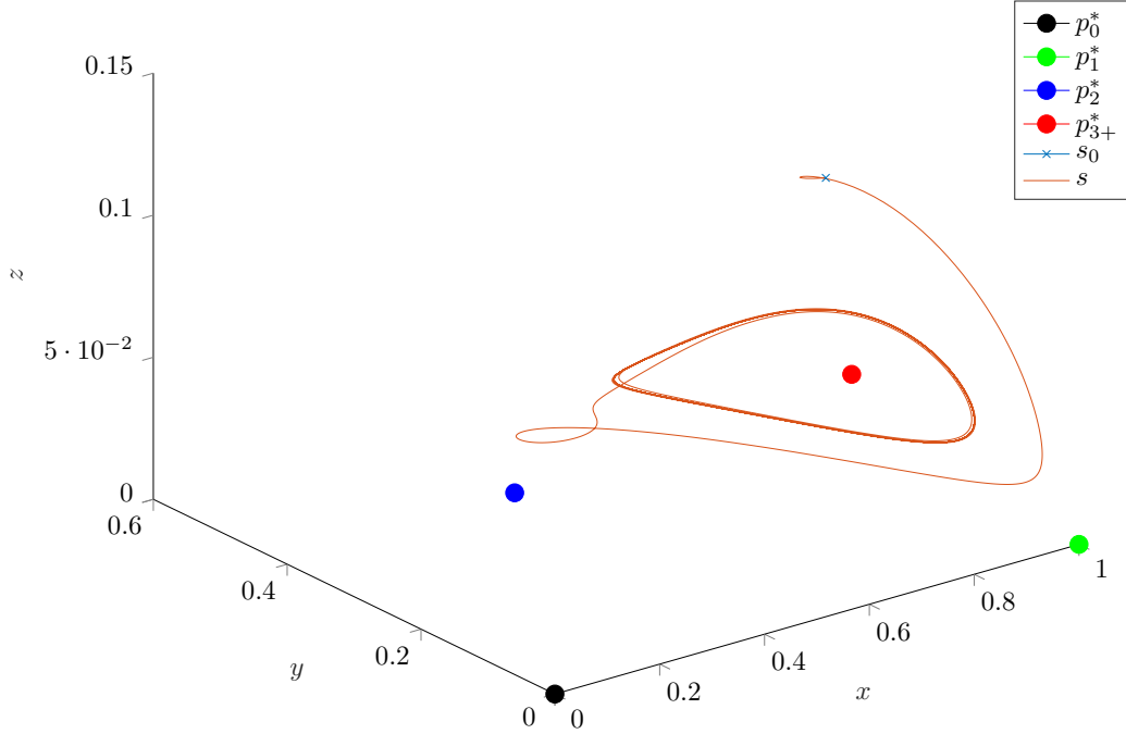
Figure 2.5.14: The limit cycle \Gamma_1^* deforms for b = 0.6
