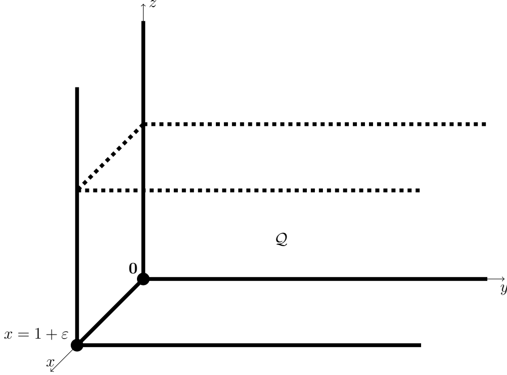
Figure 2.3.1: The set \mathcal{Q} from Lemma 2.3.2.
