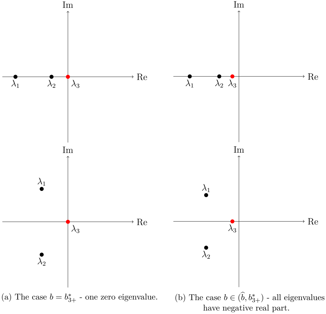
Figure 2.4.20: Constellations of \lambda_1, \lambda_2, \lambda_3 in the complex plane \mathbb{C} for b \in (\hat{b}, b_{3+}^*] .
