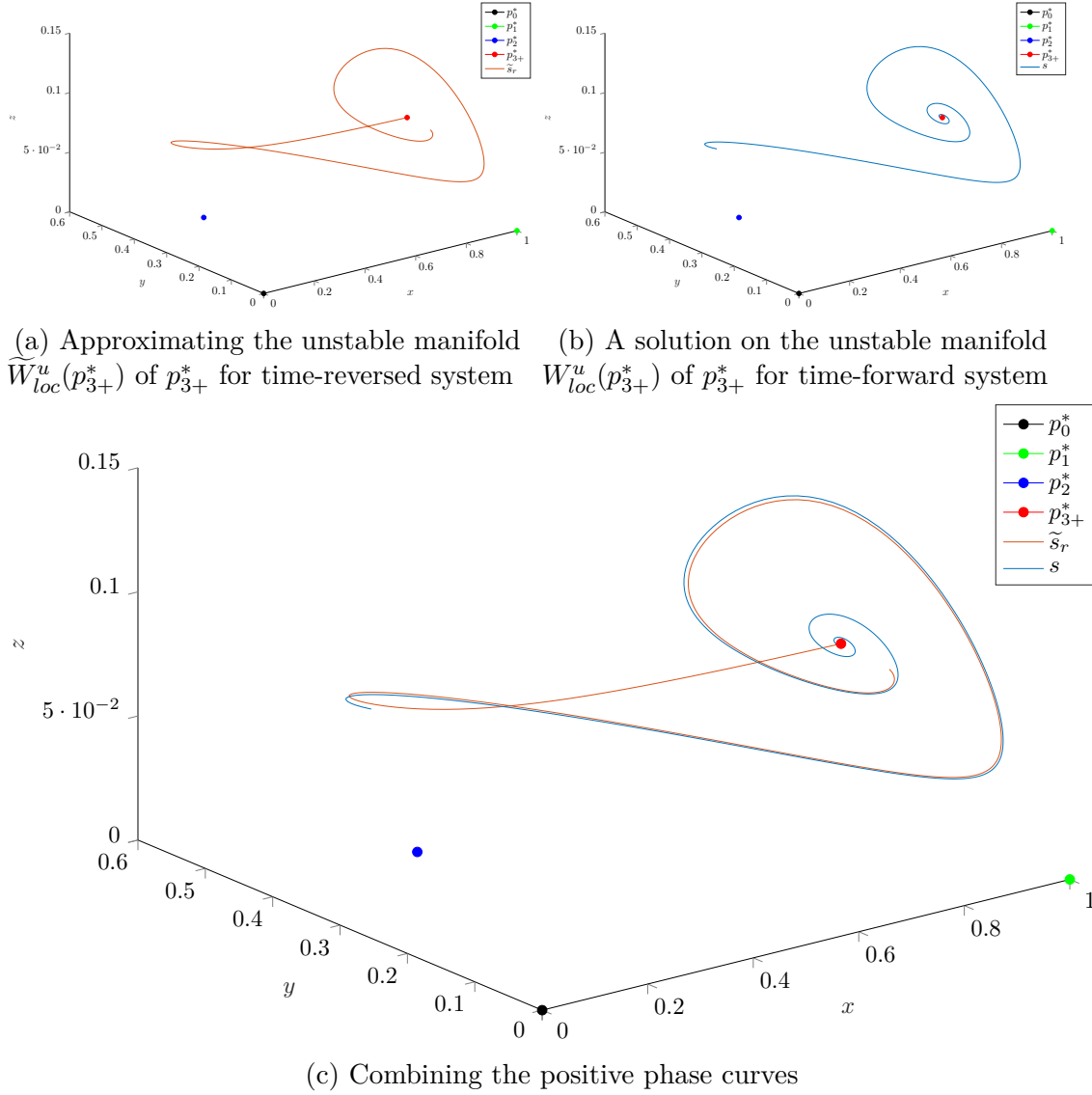
Figure 2.5.23: Solutions on the unstable manifolds of the time-forward and time-reversed system for b = 0.49964510020384728 .
