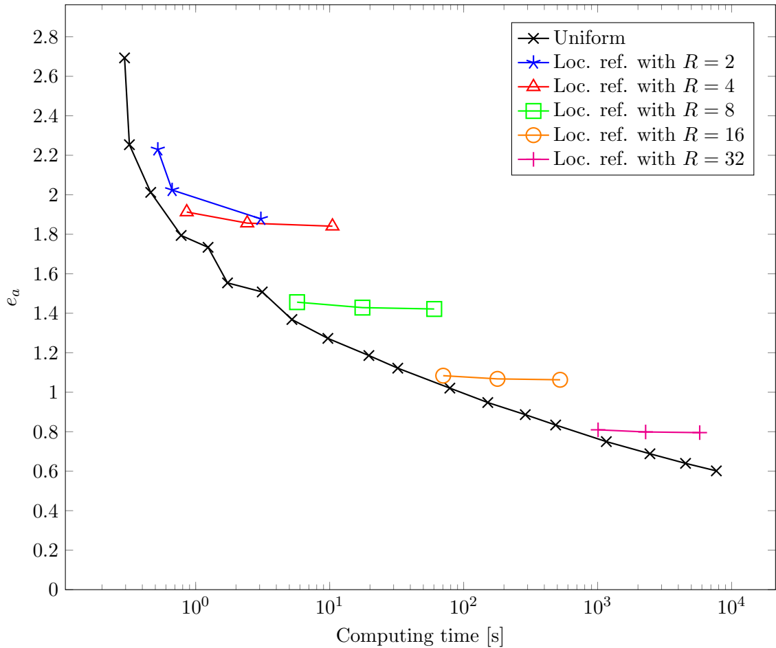
Figure 6.4: Computing times compared to the absolute pressure errors for both uniform and local refinement at the point source. Here, the plot points for all local refinement experiments indicate a change of \nu to 2, 4 and 8 from the leftmost mark to the rightmost mark. As expected, by increasing the uniform resolution R , the computing time increases inversely proportional to the error. With local refinement, however, the error is virtually unchanged, while the computing time increases noticeably. Note, that the best results for local refinement can be observed with R = 2 . But this is most likely due to the refined parts covering a large fraction of the domain and especially the spherical wave (see Figure 6.3).
