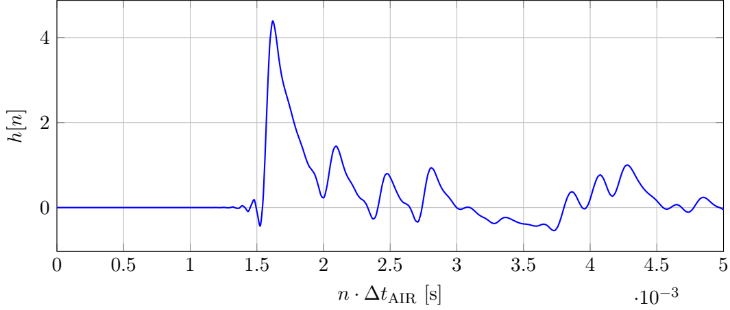
Figure 5.1: AIR for a domain of size \vec{S} = (1, 1, 1) with sample frequency f_s = 44100 Hz, receiver point P_R = (0.5, 0.5, 0.5) , source point P_S = (0.1, 0.2, 0.3) , speed of sound c_0 \approx 343 m/s and convergence order O = 4 . Impedance boundary conditions were imposed on all domain borders with reflection factor C_R = 0.5 . The source function f(t) has been simulated with T = 0.0005 . Note, that the distance between receiver and source is \|P_R - P_S\|_2 \approx 0.54 m, such that the first incidence of the wave is correctly expected after 0.54/343 \approx 1.57 \cdot 10^{-3} seconds.
