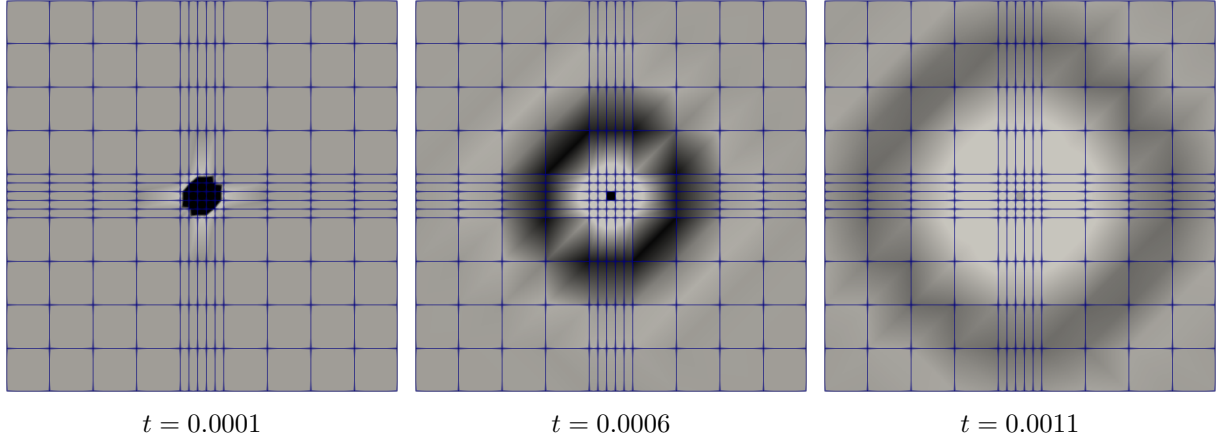
Figure 4.3: Simulation of a wave in a domain of size \vec{S} = (1, 1, 1) , which has an higher resolution around the point source P_S = (0.5, 0.5, 0.5) . For better visibility of the grid, this simulation has been executed with relatively small resolutions R = 9 and R_{P_S} = 5R = 45 . The grid is visualized using ParaView.
