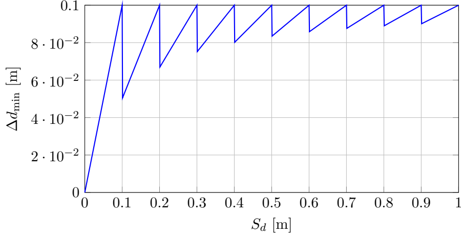
Figure 4.1: Cell widths in a uniformly discretized domain with resolution R = 10 , depending on the length S_d of the domain in one dimension d .
