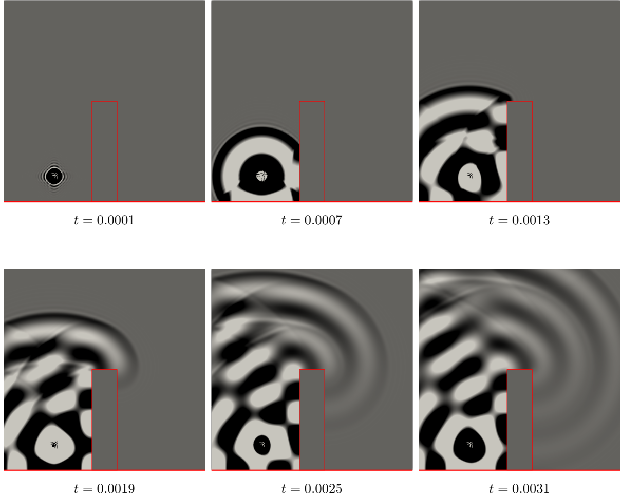
Figure 7.1: Simulation of an acoustic signal in an open environment with a totally reflecting ground and wall at the center. The domain has a size of \vec{S} = (1, 1) and the wall is 0.5 meters tall and 0.125 meters wide. The point source is located left from the wall at P_S = (0.25, 0.125) and emits sine waves with frequency 2000 Hz. It can be seen, that the source signal gets diffracted around the upper edges of the wall, such that it can still be received on the other side of the wall, as we are expecting it. Note, that all domain borders, except the ground, are absorbing. That is, with a geometric approach alone, as described in the introductory chapter 1, a receiver point right from the wall could not be backtraced to the source point by reflections only.
