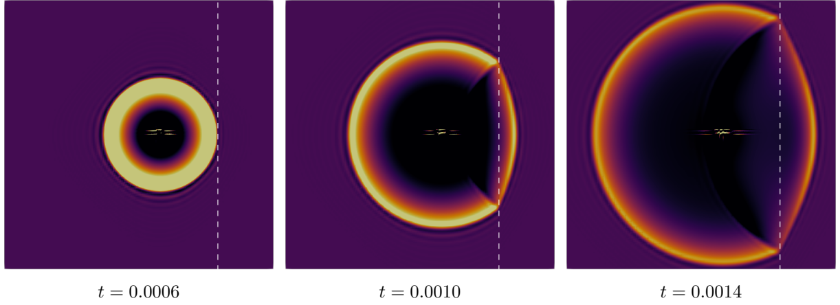
Figure 2.3: Simulation of a wave generated by a point source that is refracted at the interface between two mediums (indicated by the dashed line). The medium coefficient matrices A_i were initialized in such a way, that in the left medium, the speed of sound and impedance are c_l \approx 343 m/s and Z_l \approx 413 , whereas the wave speed in the right medium is c_r \approx 171 m/s with impedance Z_r \approx 205 . As can be seen, the wave propagating in the right medium has approximatively half the speed as in the left medium. Note also, that both, the reflected and transmitted wave, have less power than the original wave.
