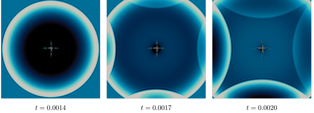
Figure 3.3: Partially reflecting boundary conditions imposed on the upper and right boundaries. In order to see the difference, total reflection is imposed on the other boundaries. The local matrices (3.24) have been set to establish a reflection coefficient of C_R = 0.2 . Note, that the wave front after the reflection does not change, i.e. the strength of the reflected wave is independent on the angle of incidence, as opposed to Figure 3.1.
