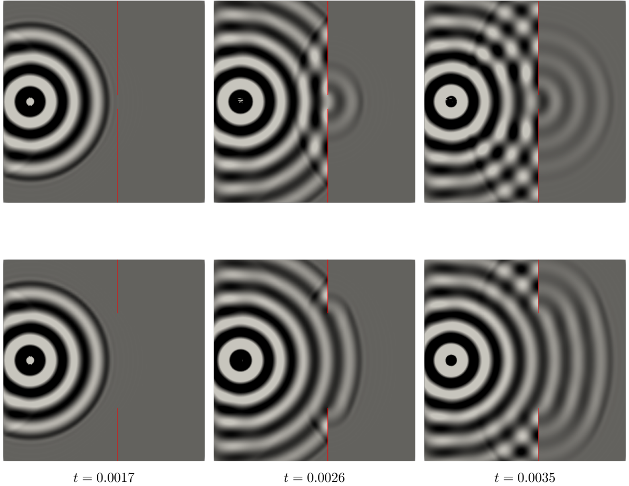
Figure 4.2: Simulation of sine waves that pass an aperture of width 0.1 m in the upper row and an aperture of width 0.6 m in the lower row. The domain has size \vec{S} = (1.5, 1.5, 1.5) , with absorbing boundary conditions imposed on all borders and a totally reflecting wall indicated by the red lines at x = 0.85 . In both scenarios, the point source is located at P_S = (0.2, 0.75, 0.75) and emits a sinusoidal signal with a frequency of 2000 Hz. The wave speed is \approx 343 m/s. These illustrations show a two-dimensional slice of the domain at z = 0.75 . As can be seen in both simulations, the waves hitting the aperture get diffracted around the corners into the so-called acoustic shadow [1, sec. 7.2.3].
