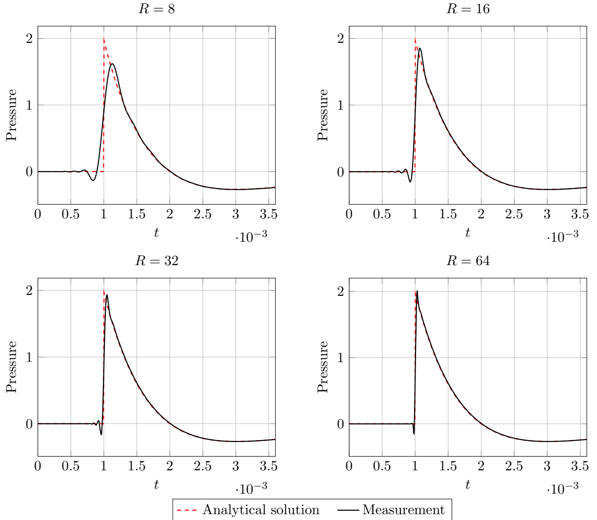
Figure 6.2: AIR measurements compared to the analytical solution for different R . The receiver point has been chosen to be located at P_R = (1.698, 1.698, 1.698) , such that the distance to the source is \|P_R - P_S\|_2 = \sqrt{3 \cdot 0.198^2} \approx 0.343 meters. Hence, the wave arrives at the receiver after \approx 0.343/343 = 1 \cdot 10^{-3} seconds.
