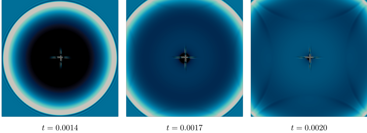
Figure 3.1: Simulation of a wave in a 1 \times 1 \times 1 -meter domain with absorbing boundary conditions imposed on all borders of the domain. A point source in the center radiates a wave with velocity \approx 343 m/s, which thus hits the boundaries after \approx 0.0015 seconds. These illustrations show a slice of the three-dimensional space in x - y -plane at z = 0.5 . As can be seen in the middle and right image, the wave is mostly absorbed, but weak ingoing waves still arise. Note, that the strengths of those ingoing waves vary with the angle. A wave hitting the border frontally just advects along a single dimension and can thus be totally absorbed. But the steeper the angle of incidence is, the stronger is the wave that arises at the boundary, which can be seen in the right image.
