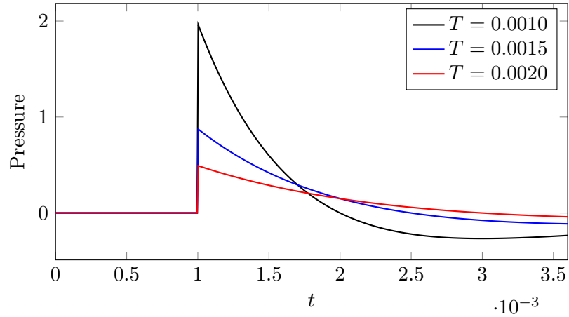
Figure 6.6: Analytical solutions for the pressure magnitude of the AIR with different T . The distance between receiver and source is \approx 0.343 meters.
