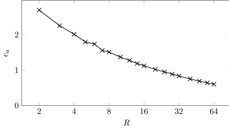
Figure 6.1: Absolute pressure errors depending on the global resolution R for uniform refinement.
