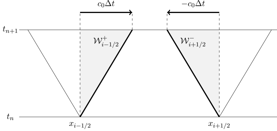
Figure 2.2: Waves propagating from the left ( x_{i-1/2} ) and right ( x_{i+1/2} ) cell interfaces. Q_i^n is updated by the waves \mathcal{W}_{i-1/2}^+ and \mathcal{W}_{i+1/2}^- reaching into cell \mathcal{C}_i after time \Delta t . This illustration is based on [3, p. 79, Fig. 4.7].
