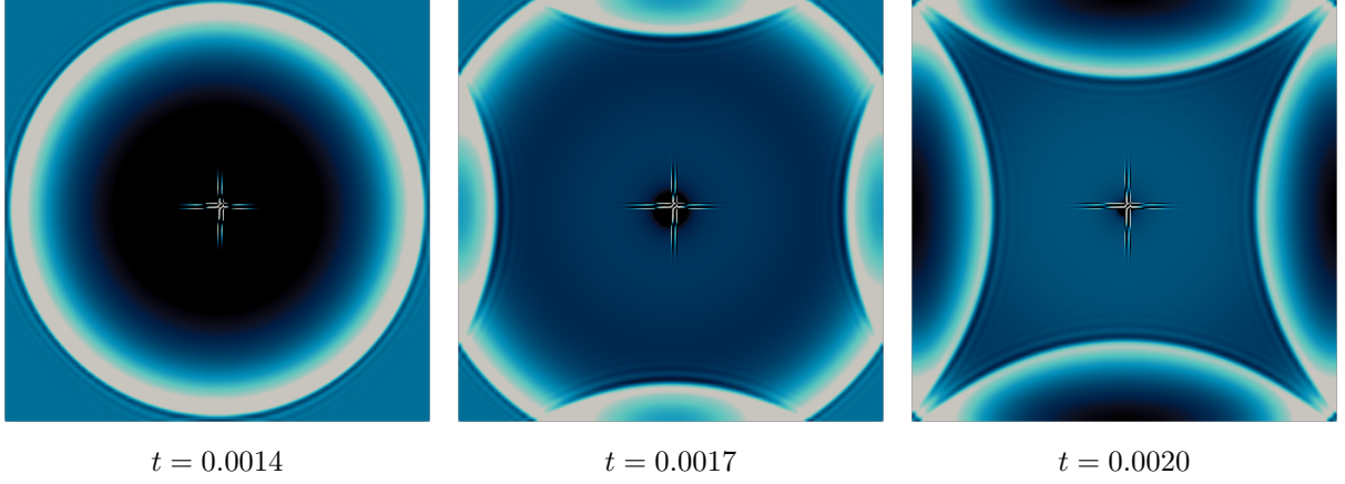
Figure 3.2: Simulation of the same wave and physical domain as in Figure 3.1, but with totally reflecting boundary conditions imposed on all borders. As can be seen in the images, the reflected waves have the exact same power as the incident waves, i.e. no energy is lost.
