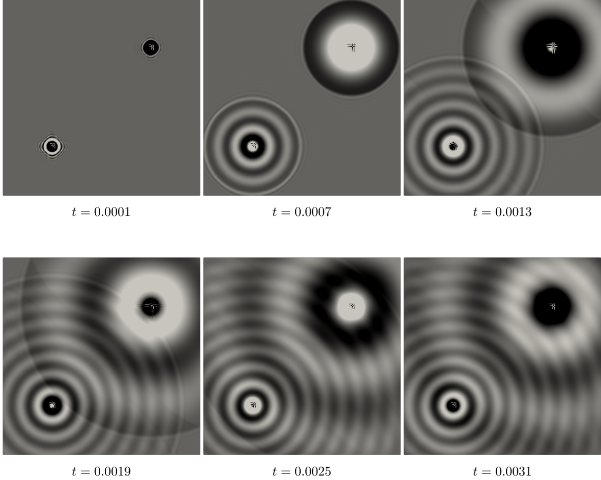
Figure 7.4: Simulation of two simultaneous point sources at \vec{P}_{S1} = (0.25, 0.25) and \vec{P}_{S2} = (0.75, 0.75) in a domain of size \vec{S} = (1, 1) . The former signal is a cosine with frequency 4000 Hz and a maximal amplitude of 0.1, whereas the latter source emits a sinusoidal signal with a frequency of 1000 Hz and a maximal amplitude of 1. In fact, the simulation system has been extended to allow for arbitrarily many individual point sources. This could be, for instance, useful for convolution reverberation, if it is known beforehand that the same source signal is always emitted at various points in the environment simultaneously, like in concert halls with multiple loudspeakers. In doing so, it can be avoided to measure the AIR for each source point separately. However, this would of course require to use the exact same signal (5.7), including the same T , for all sources.
