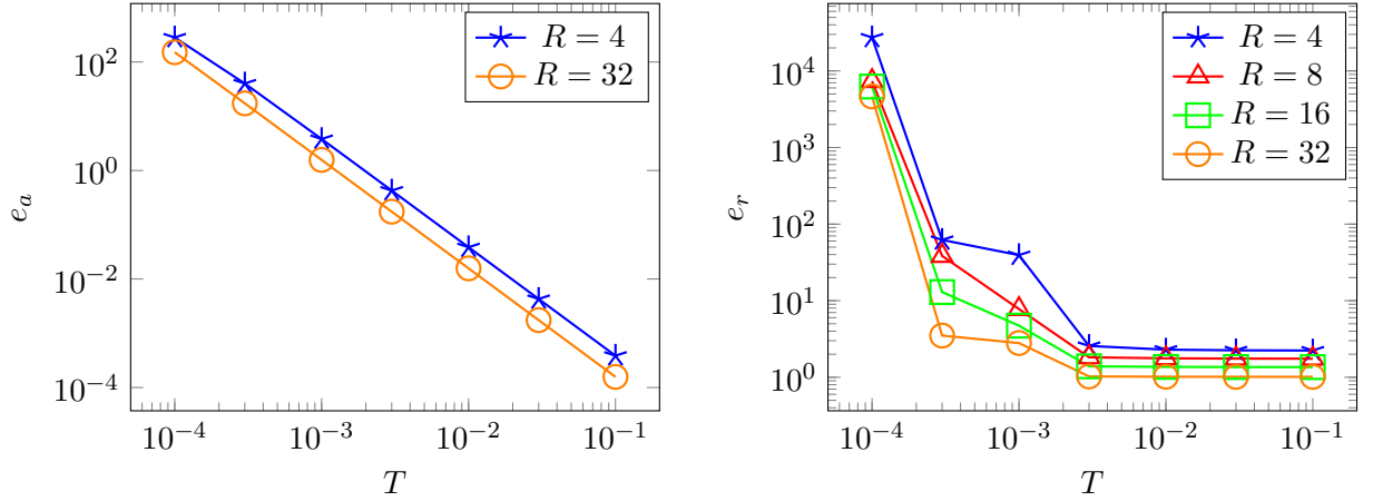
Figure 6.5: Absolute (left) and relative (right) pressure errors for different global resolutions depending on the coefficient T .
