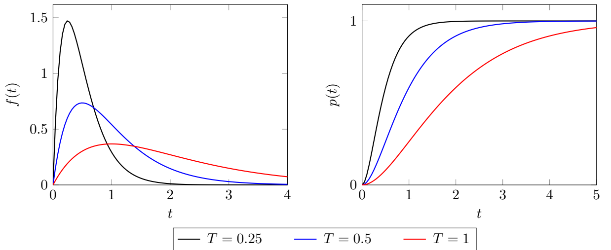
Figure 6.7: Approximative impulse (left) and its antiderivative (right) with different values for the parameter T .
