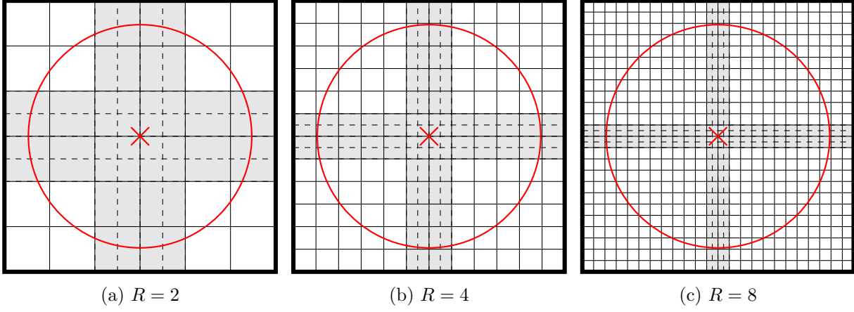
Figure 6.3: Illustration of the domain grid with size \vec{S} = (3, 3, 3) . The locally refined source point (indicated by the red cross) is located in the center of the domain at P_S = (1.5, 1.5, 1.5) , where \nu = 2 holds for each of the above shown grids. These illustrations show a two-dimensional slice of the domain at its center. The red circle displays the wave front at the end of the simulations after t_{\text{sim}} = 0.0036 seconds. Note, that the volume of the locally refined parts of the domain (here indicated by the gray areas) decreases, the higher R is. This is because the source point can already be isolated better with higher global resolutions.
