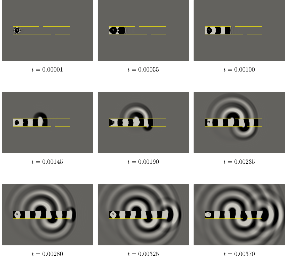
Figure 7.2: Simulation of an acoustic signal within an onesidedly opened pipe. Note, that, contrary to all previously presented experiments, the domain is not cubical, but has size \vec{S} = (1.5, 1) . The pipe (indicated by the yellow lines) has corner points (0.1875, 0.4375) and (1.125, 0.5625) . Moreover, it has small holes of width 0.0625 meters, once in the top of the pipe at x = 0.625 (left corner), and once in the bottom at x = 0.8125 . Partially reflecting boundary conditions have been imposed on the whole pipe with reflection factor C_R = 0.9 .
