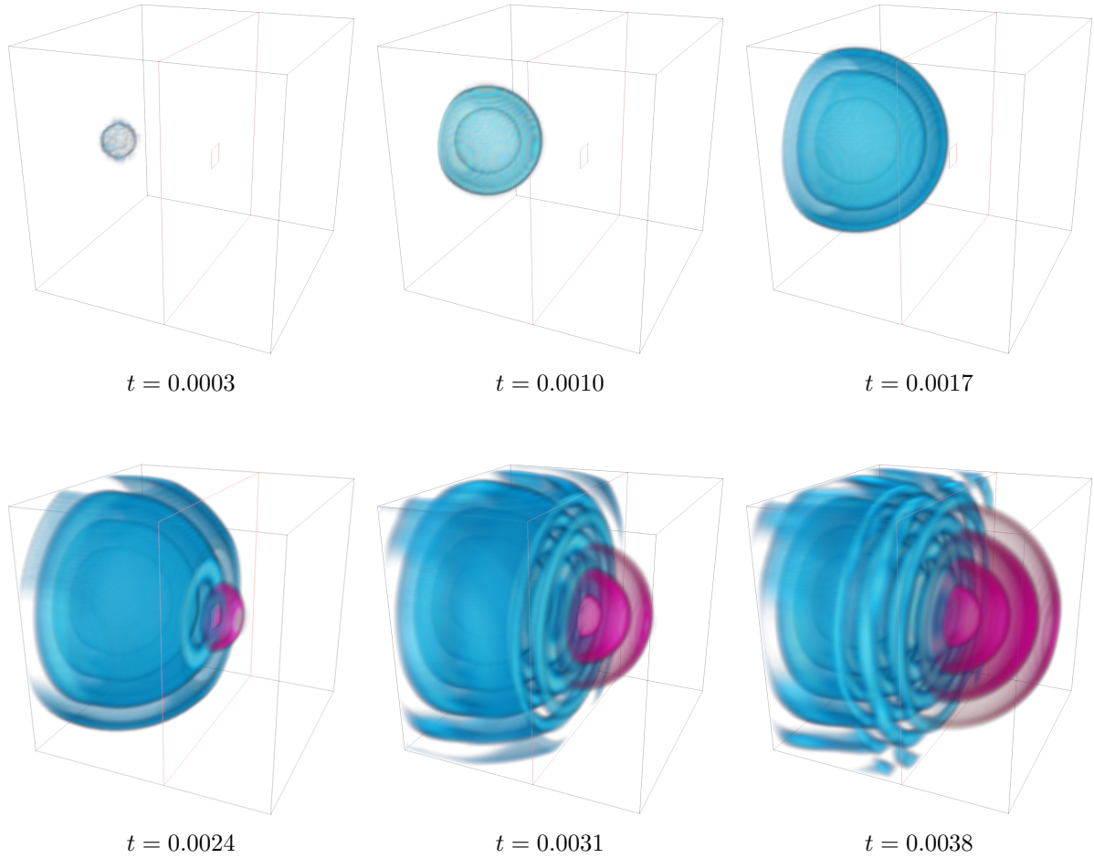
Figure 7.3: Three-dimensional simulation of a sinusoidal source signal with frequency 2000 Hz, that gets diffracted due to a small hole in a wall. The point source is located at P_S = (0.2, 0.75, 0.75) in a domain of size \vec{S} = (1.5, 1.5, 1.5) . The totally reflecting boundary lies at x = 0.875 and has a square-shaped hole in it with a width of 0.125 meters (indicated by the red slice in the center of the wall). To better distinguish the waves coming from the original source (blue) and the new spherical waves that arise at the aperture (purple), we colored the areas of the domain that are segregated by the wall differently. Note further, that for reasons of visibility, the purple color map covers a more narrow range of pressure values, as the waves behind the aperture are very weak. Thus, those waves may appear stronger than they actually are. For a better comparability of the pressure magnitudes, refer to Figure 4.2, where a similar experiment is shown in 2D.
