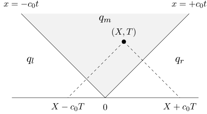
Figure 2.1: Solution of the Riemann problem for (X, T) , where one point of its DOD (indicated by the dashed lines) is left and the other one right from the initial discontinuity at x = 0 . The solution is then based on both initial states q_l and q_r , instead of just one of those. This establishes a new constant middle state q_m between the two wedges (gray area), which propagates in either direction with the speed of sound \mp c_0 . That is, the solution at each point (X, T) , for which |X| < c_0T holds, is q_m . This illustration is based on [3, p. 54, Fig. 3.3].
