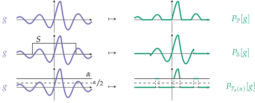
Figure 3.3: Illustration to Example 3.14 (positivity, support, amplitude thresholding projectons).
