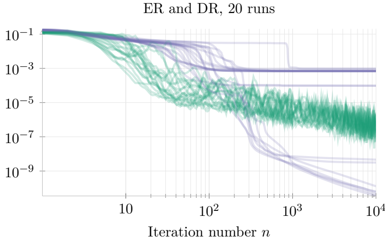
Figure 10.2: ER and DR: global rand. init.; N = 63 (Example 10.2). Energy for 20 runs of ER and DR for g_{3G,63} with random initialization, cf. Example 10.2. The energy is plotted in units of 1/\|\check{\mathbf{I}}\|_2 .
