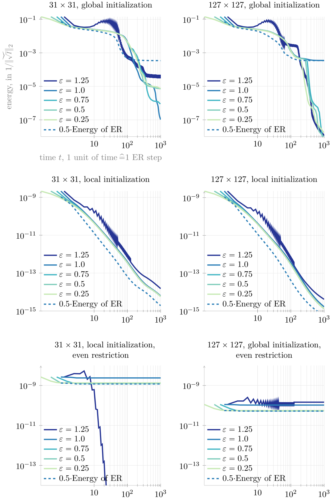
Figure 10.7: Similar dynamics of ER and ERF (see Example 10.7 ). Axis labels of the upper left graphs apply to all graphs of this figure.
