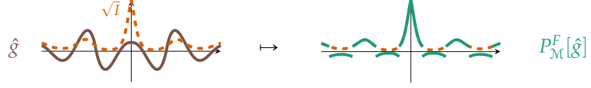
Figure 3.5: Illustration to Example 3.24 (modulus projection).
