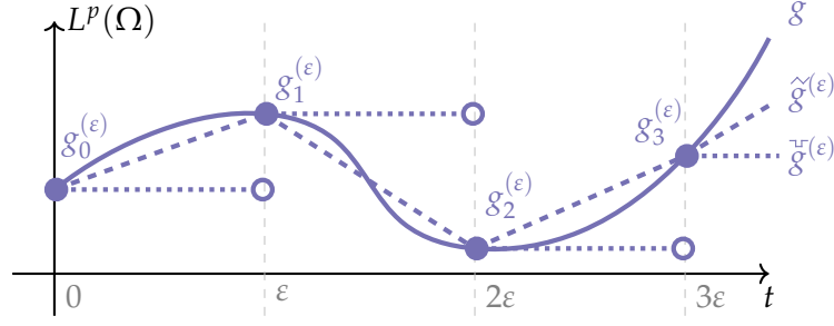
Figure 7.1: Illustration to Chapter 7 (Global solution of ERF).
