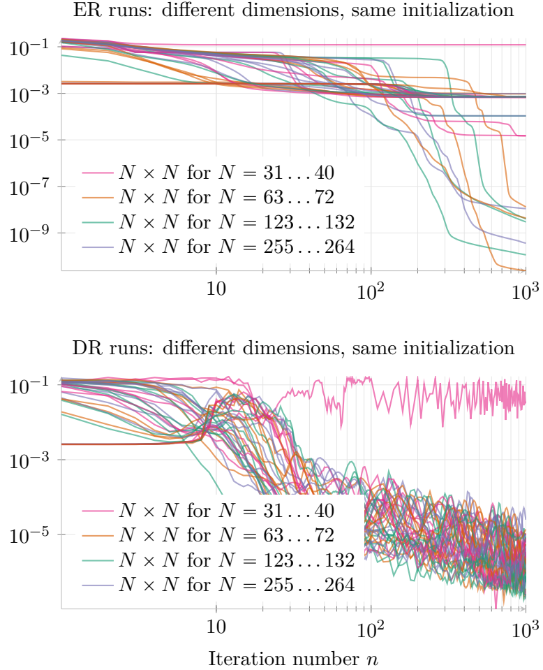
Figure 10.5: ER and DR: global zero phase init.; different N (Example 10.5).
