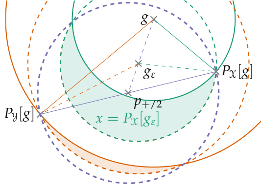
Figure 6.1: Illustration to Proposition 6.8 (dAPF does not increase projection difference).
