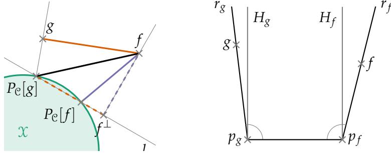
Figure 5.2: Illustration to Proposition 5.21 and Lemma 5.22 (subdifferentials of convex energy functionals).
