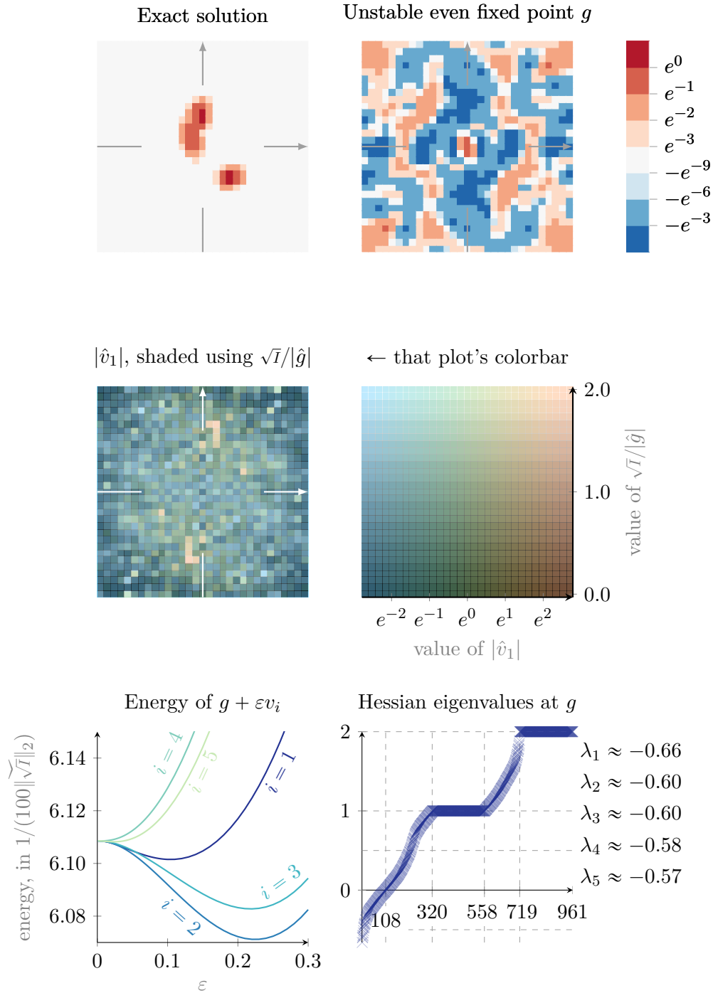
Figure 10.10: The Hessian: unstable FP far from solution (see Example 10.10 ).
