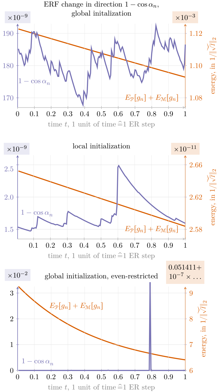
Figure 10.9: Direction change of ERF (see Example 10.9 ). The plots depict the quantity 1 - \cos \alpha_n , where the cosine angle is the angle between two consecutive updates, see Example 10.9 . One can see that — also for the even-restricted case, where the algorithm converges to a fixed point (implied by the energy decay) — the algorithm changes the direction in a discontinuous manner.
