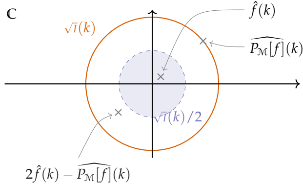
Figure 8.2: Illustration to Corollary 8.2 (ER fixed point correspondence).
