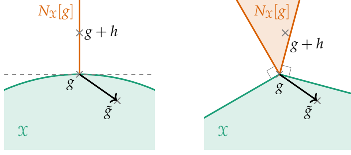
Figure 5.3: Illustration to Definition 5.30: normal cones to convex sets. Two examples of convex cones N_X to convex set X at g \in X . For any h \in N_X , the angle between \hat{g} - g and (g + h) - g is greater or equal than \pi/2 for all \hat{g} \in X , i.e. \langle \hat{g} - g, h \rangle \leq 0 . On the left, N_X[g] given by a ray; on the right, N_X[g] has non-empty interior.
