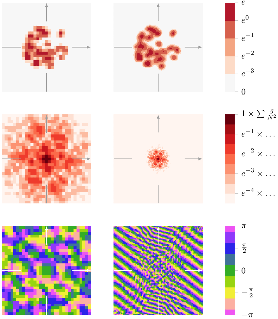
Figure E.3: Sum of 27 Gaussians
