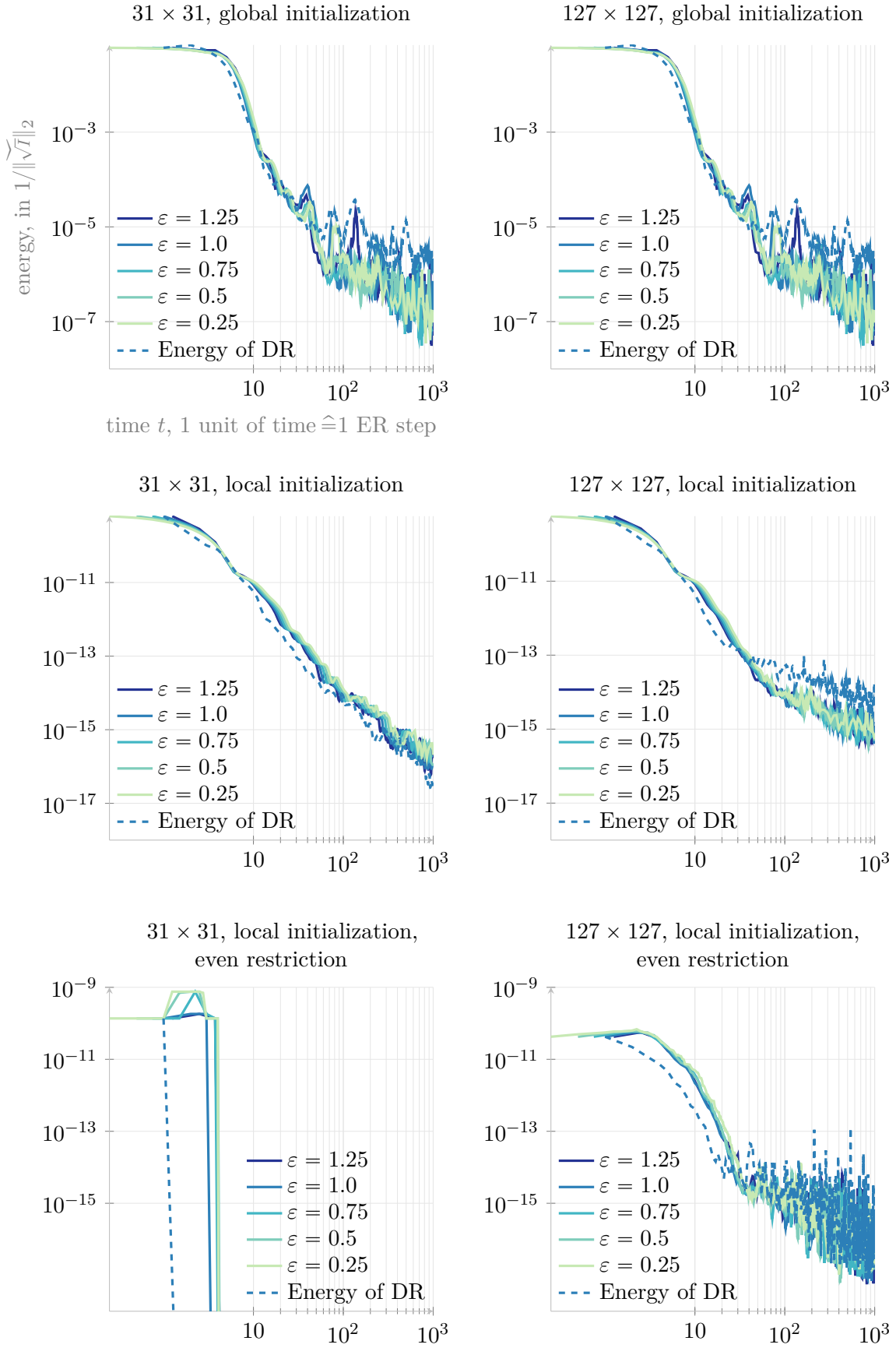
Figure 10.8: Similar dynamics of DR and DRF (see Example 10.8 ). Axis labels of the upper left graphs apply to all graphs of this figure.
