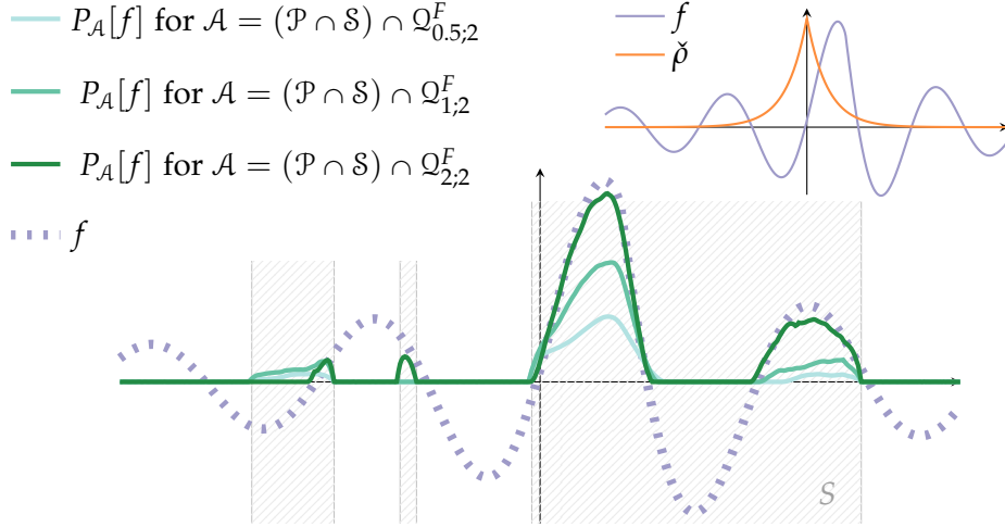
Figure 6.2: Illustration to Remark 6.42 (regularized \mathcal{P} \cap \mathcal{S} ).
