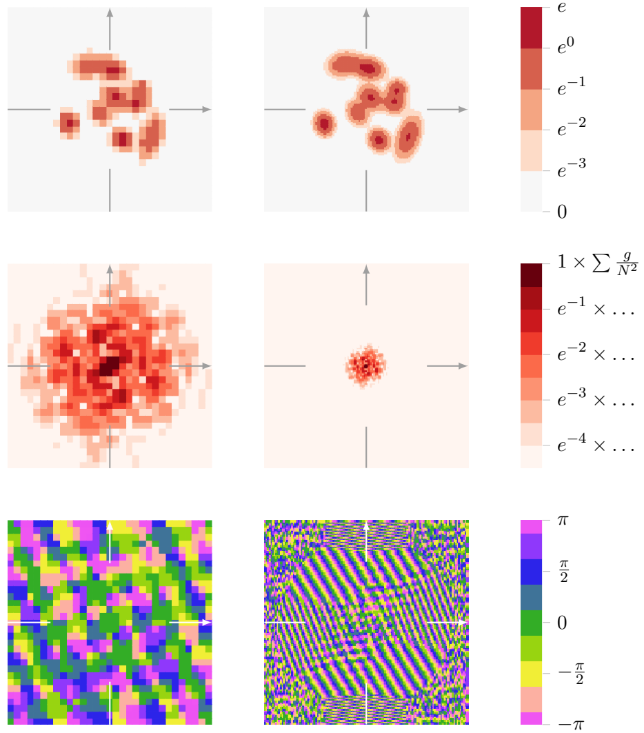
Figure E.2: Sum of 9 Gaussians from Table E.2
