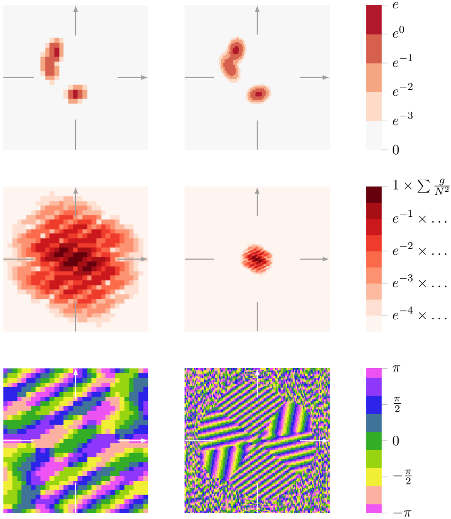
Figure E.1: Sum of 3 Gaussians from Table E.1
