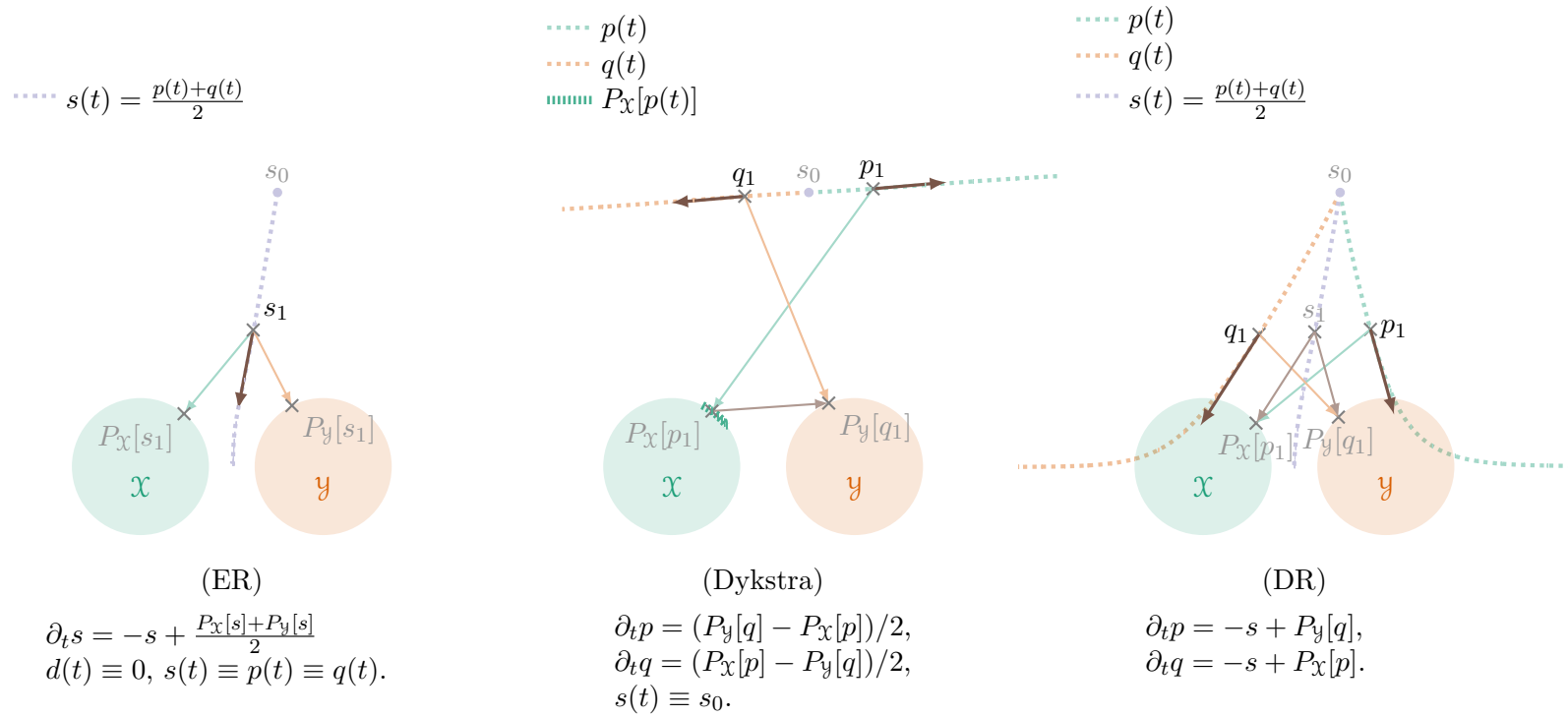
Figure 9.2: Updates of discretized 2v-FPF (Example 9.10)
