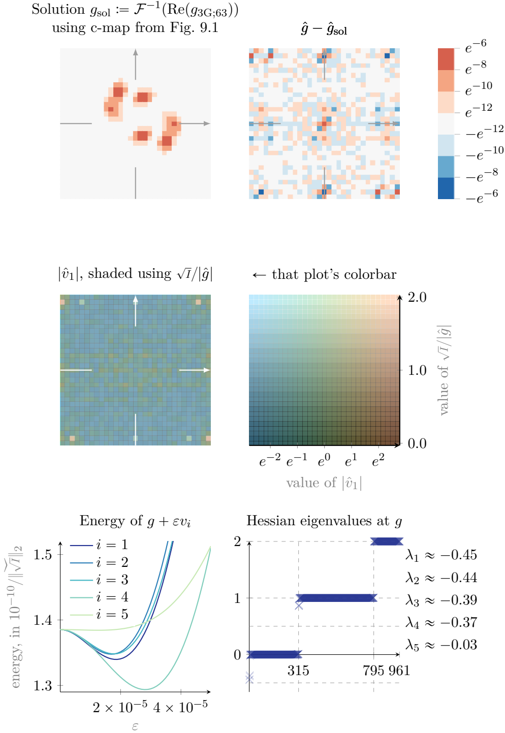
Figure 10.12: The Hessian: unstable FP near solution (see Example 10.12 ).
