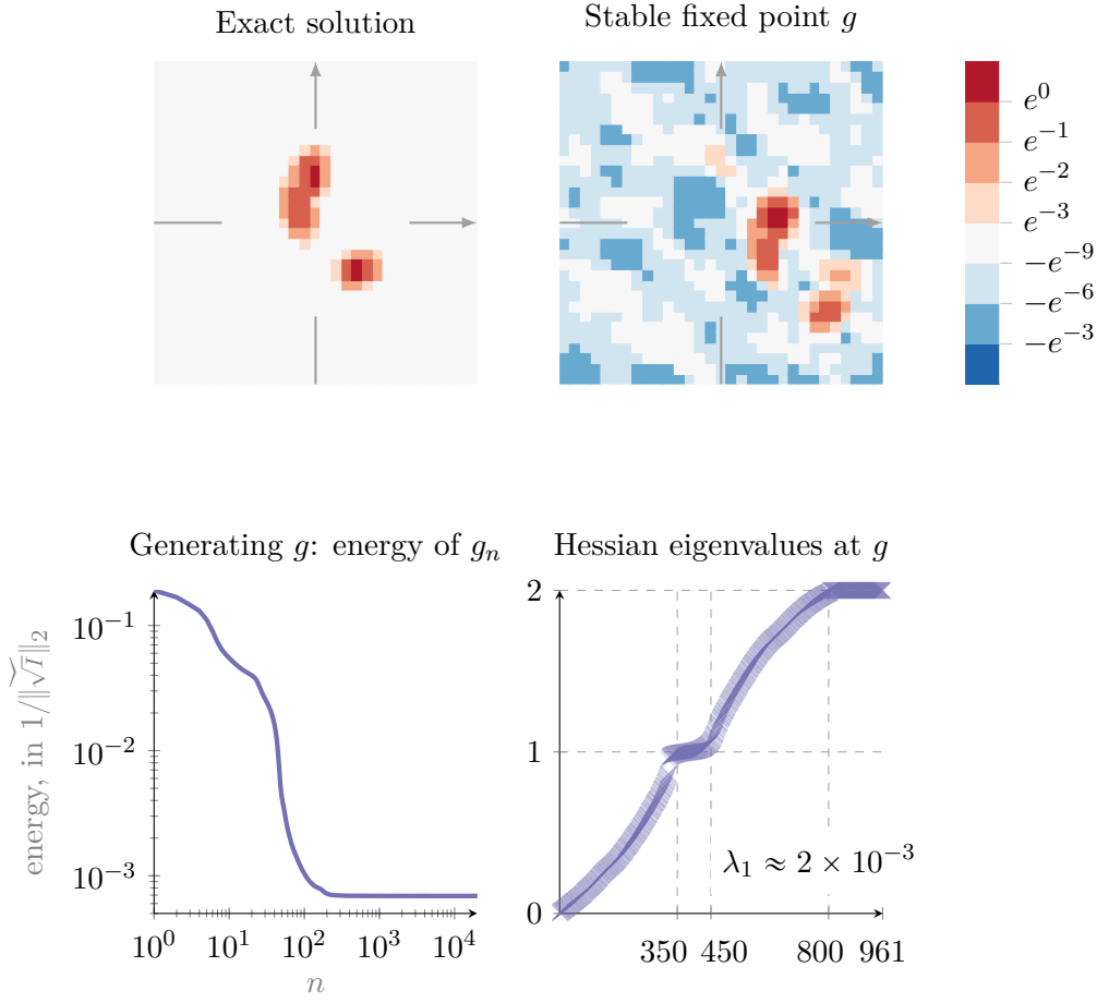
Figure 10.11: The Hessian: stable FP (see Example 10.11 ).
