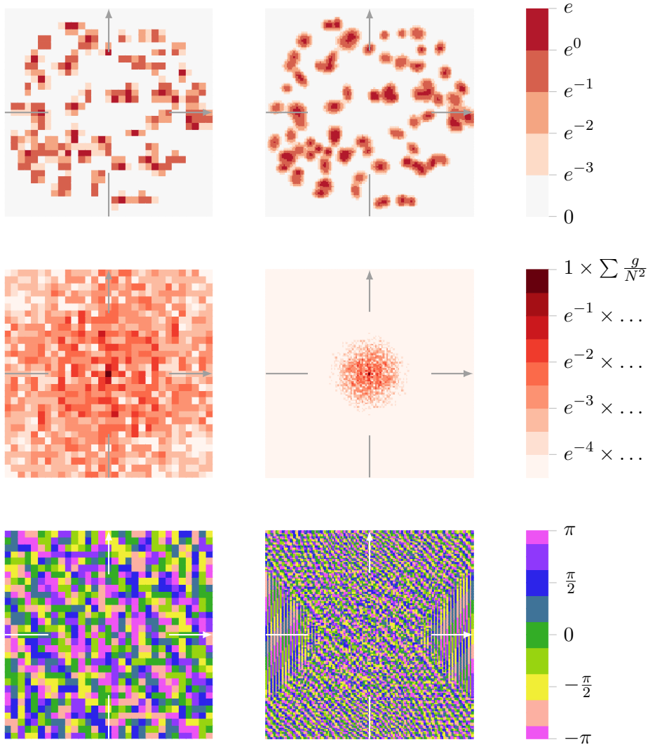
Figure E.5: Sum of 84 Gaussians, large support radius Top left: g_{84G;31} . Top right: g_{84G;127} . Center left: |\hat{g}_{84G;31}| . Center right: |\hat{g}_{84G;127}| . Bottom left: \arg(\hat{g}_{84G;31}) . Bottom right: \arg(\hat{g}_{84G;127}) . Graphs of phases are modulated by e^{ix_0} , where the shift x_0 is approximately equals to the barycenter of the corresponding function (to minimize visual cluttering due to phase oscillations). In comparisson to concentrated Gaussians (Figure E.4), solution phase (in the bottom row) is notably less regular.
