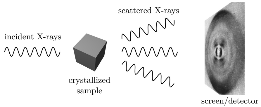
Figure 1.1: Sketch of a crystallographic measurement.
