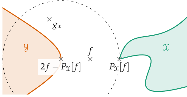
Figure 8.1: Illustration to Proposition 8.1 (Fixed points of AP and APF).
