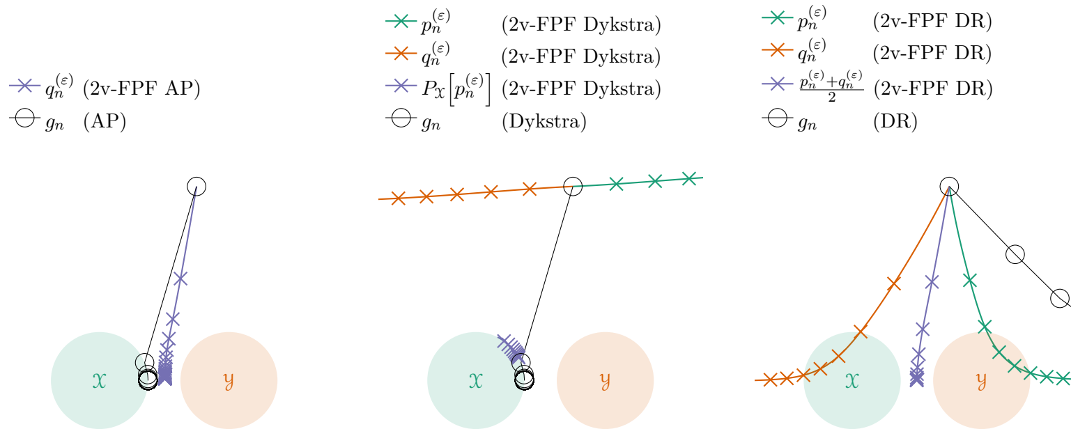
Figure 9.4: Dynamics of 2v-FPF AP, Dykstra and DR: non-feasible convex case
