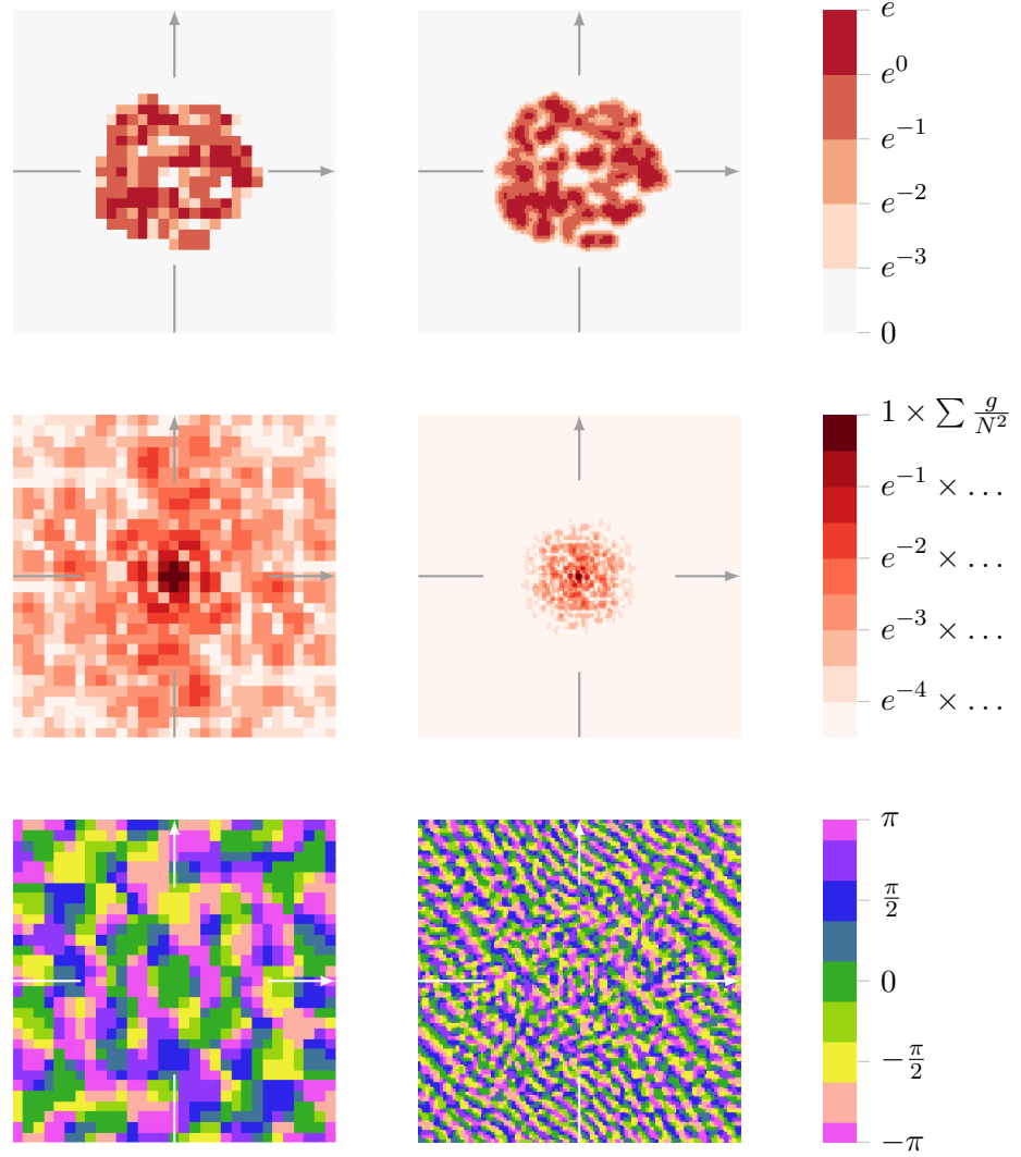
Figure E.4: Sum of 84 Gaussians
