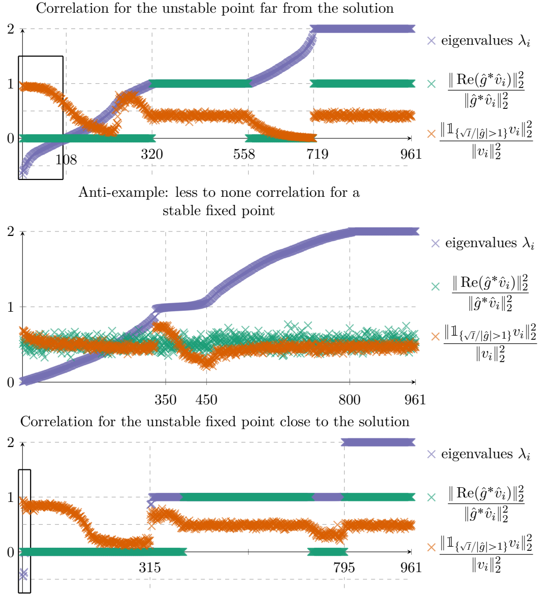
Figure 10.13: Eigenvector correlations for unstable fixed points (Example 10.13).
