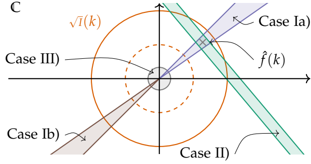
Figure 8.3: Illustration to Remark 8.8 (Interpretation of \widehat{P}_{\mathcal{M}} at k ). Dashed orange circle is of radius \sqrt{I(k)}/2 .
