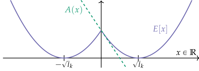
Figure 4.1: Illustration to Example 4.26 (Slope of the modulus energy). The function E[x] = \frac{1}{2}(|x| - \sqrt{I_k})^2 is non-differentiable at the point x = 0 . Its slope at 0 equals \sqrt{I_k} (cf. the tangent A(x) = -\sqrt{I_k}x + \frac{1}{2}\sqrt{I_k}^2 ).
