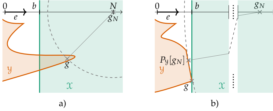
Figure 9.1: Illustration to Proposition 9.7 (half-space feasibility problem).
