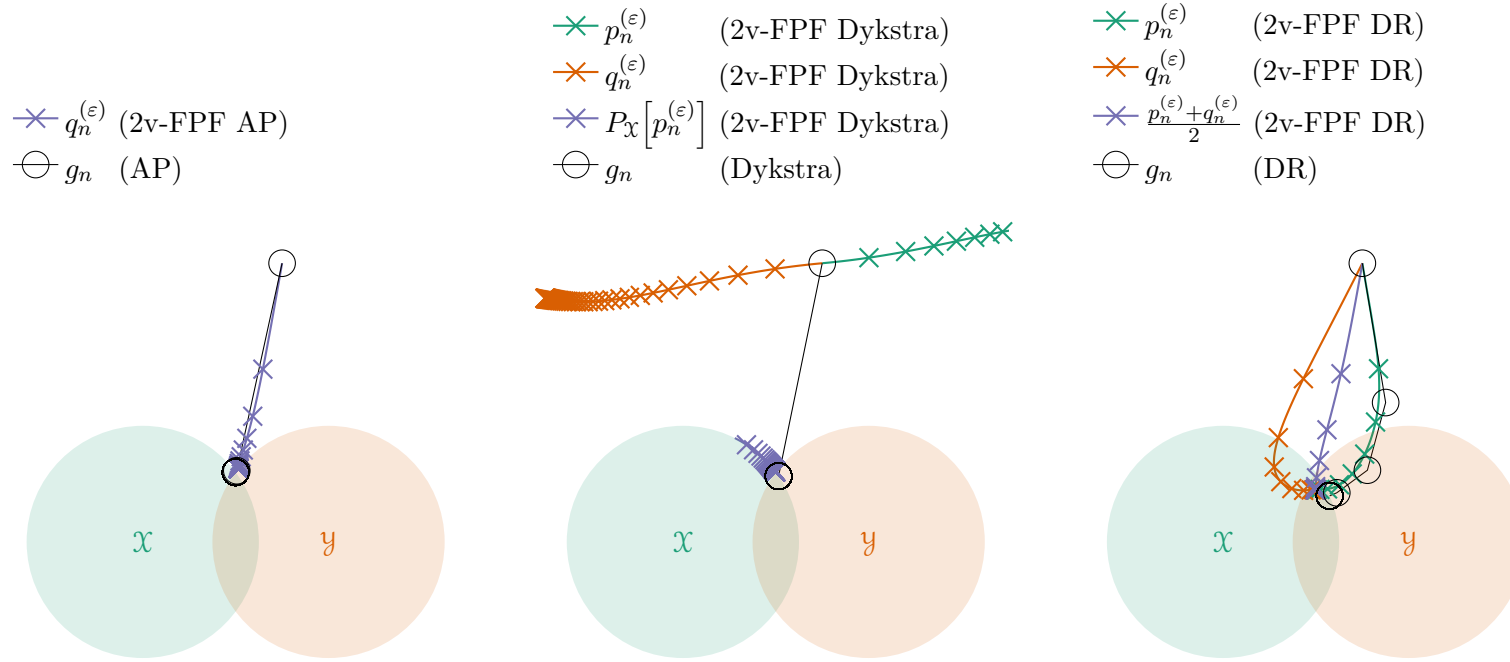
Figure 9.3: Dynamics of 2v-FPF AP, Dykstra and DR: feasible convex case
