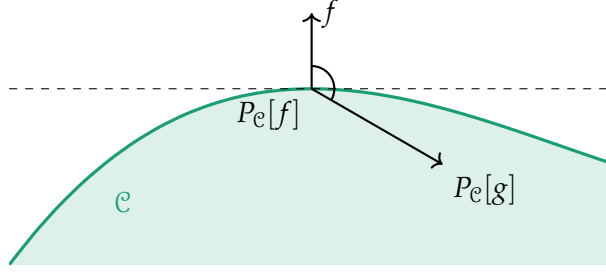
Figure 3.2: Illustration to Lemma 3.10 (angle property for convex projectors). For a convex set \mathcal{C} , the angle between f - P_{\mathcal{C}}[f] and P_{\mathcal{C}}[g] - P_{\mathcal{C}}[f] is larger than \pi/2 for any g \in \mathcal{H} , i. e. \langle f - P_{\mathcal{C}}[f], P_{\mathcal{C}}[g] - P_{\mathcal{C}}[f] \rangle \leq 0 .
