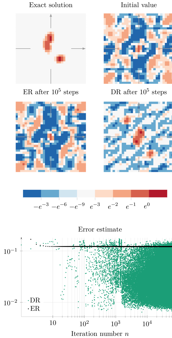
Figure 10.6: ER and DR: a non-converging run (Example 10.6). ER and DR for g_{3G,31} with the zero phase initialization, cf. Example 10.6. The energy is plotted in units of 1/\|\check{\sqrt{I}}\|_2 . The algorithms do not converge after 10^5 iterations.
