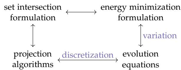
Figure 1.2: Various formulations of phase retrieval.
