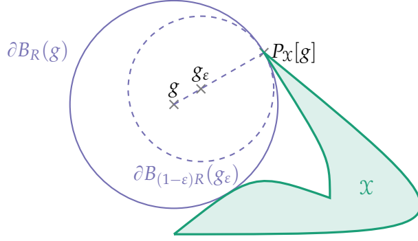
Figure 3.1: Illustration to Lemma 3.8 (interpolation projecton property). One has P_X[g_\epsilon] = P_X[g] , even if the set \arg \min_{f \in X} \|g - f\|_2 contains more than one element.
