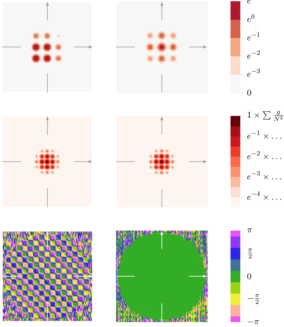
Figure B.1: Non-uniqueness of solutions (Example B.3)
