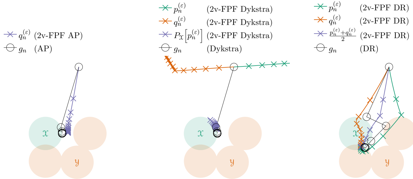
Figure 9.5: Dynamics of Dv-FPF AP, Dykstra and DR: feasible non-convex case
