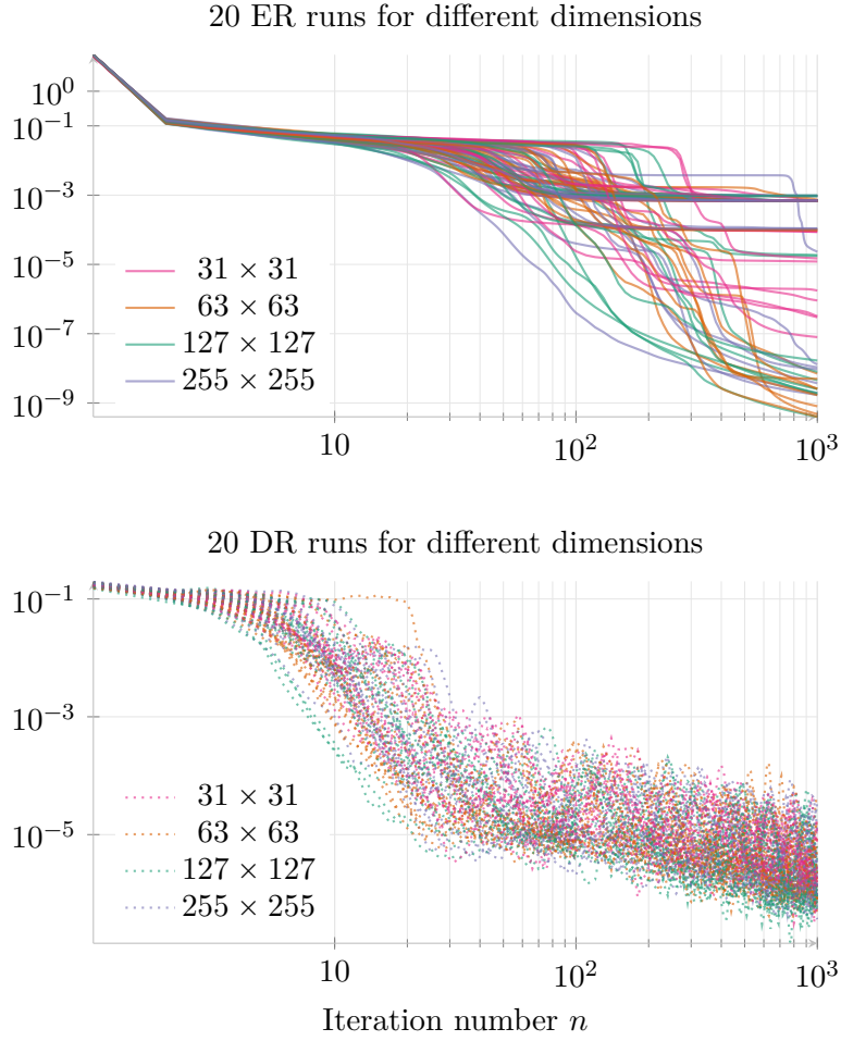
Figure 10.4: ER and DR: global rand. init.; N \in \{31, 63, 127, 255\} (Example 10.4).
