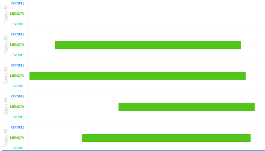
Figure 5.5.: Example of multiple command queues in one device.
