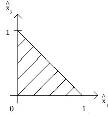
Abbildung 6.4: Standardelement \hat{T} := \{\hat{x} \in \Omega : \hat{x}_1, \hat{x}_2 \geq 0, \hat{x}_1 + \hat{x}_2 \leq 1\}
