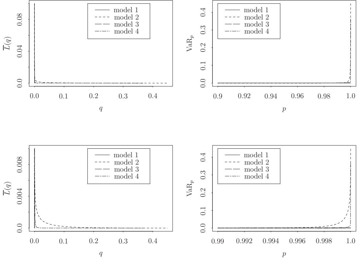
Figure 5.1: Tail-distribution and Value-at-Risk of the four models with group A -parameter setting.
