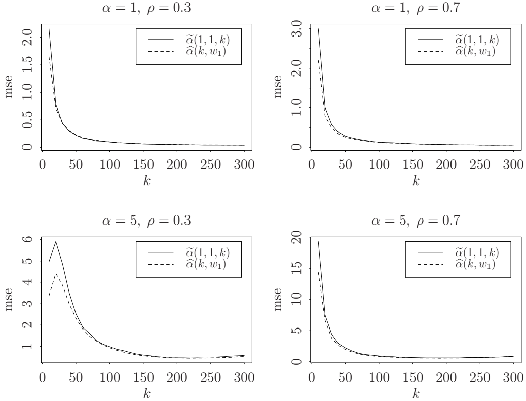
Figure 3.4: Estimated mean squared errors of estimators in Figure 3.3.
