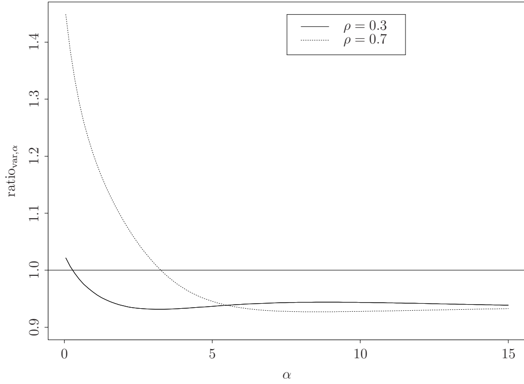
Figure 3.1: Theoretical ratios, \text{ratio}_{\text{var}, \alpha} , are plotted against \alpha for \rho = 0.3 and 0.7 .
