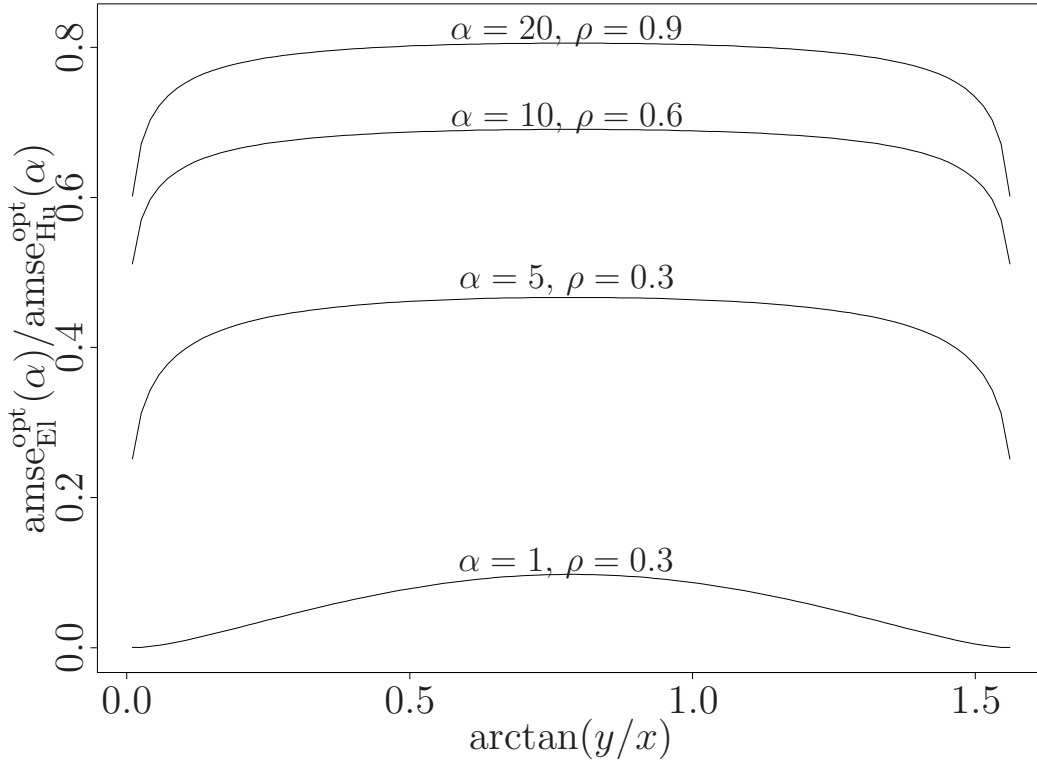
Figure 2.4: Ratio \text{amse}_{\text{El}}^{\text{opt}}(\alpha)/\text{amse}_{\text{Hu}}^{\text{opt}}(\alpha) , x^2 + y^2 = 2 , for different (\alpha, \rho) and \beta = -1 .
