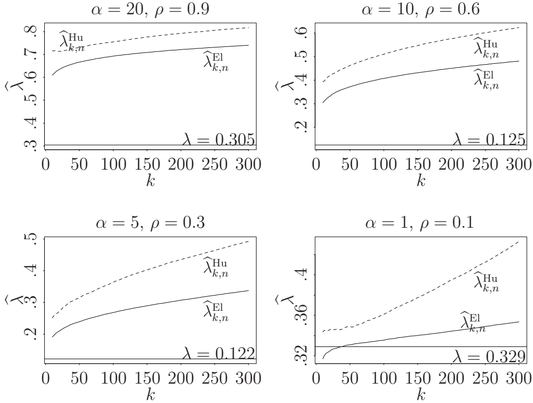
Figure 2.6: Mean of estimators \hat{\lambda}_{k,n}^{\text{Hu}}(1,1) and \hat{\lambda}_{k,n}^{\text{El}}(1,1) for 1000 samples of length n = 1000 and different k with \sigma = v = 1 , \boldsymbol{\mu} = \mathbf{0} , G \sim \text{Pareto}(\alpha) and different (\alpha, \rho) .
