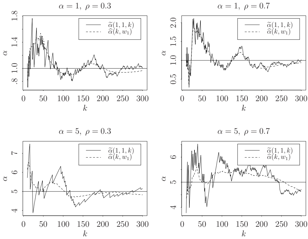
Figure 3.7: Estimators \tilde{\alpha}(1, 1, k) and \hat{\alpha}(k, w_1) based on a particular sample are plotted against k = 10, 11, \dots, 300 .
