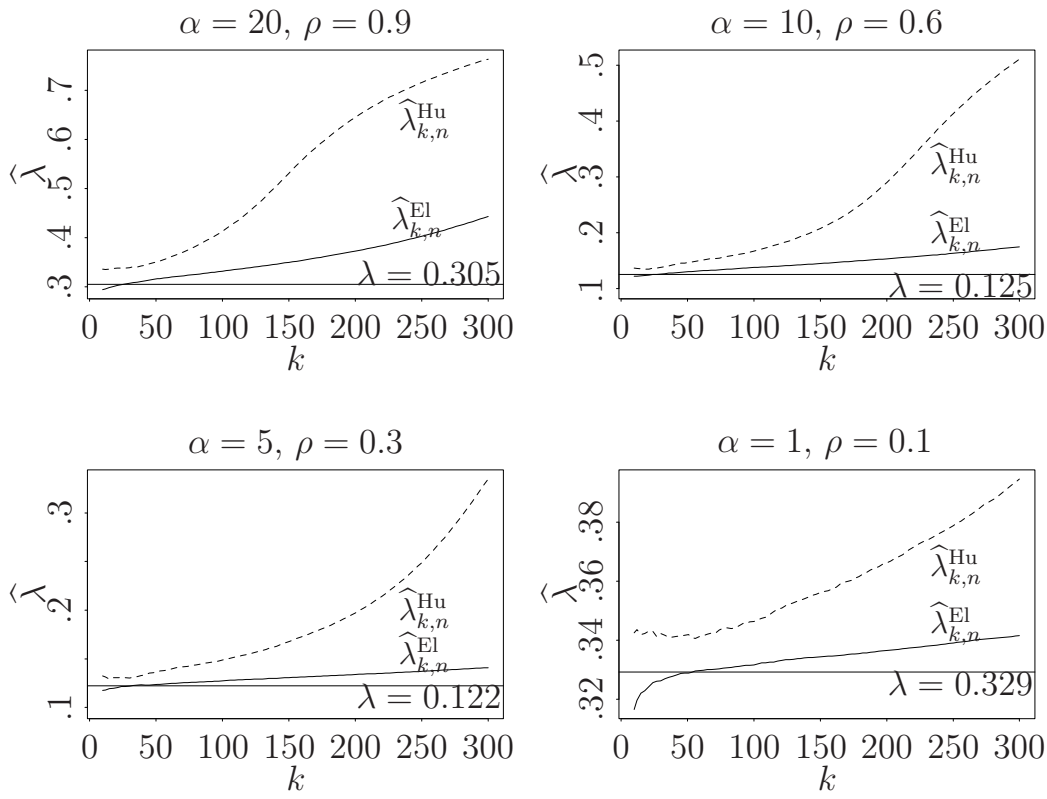
Figure 2.5: Mean of estimators \hat{\lambda}_{k,n}^{\text{Hu}}(1,1) and \hat{\lambda}_{k,n}^{\text{El}}(1,1) for 1000 samples of length n = 1000 and different k with \sigma = v = 1 , \boldsymbol{\mu} = \mathbf{0} , G \sim \text{Fréchet}(\alpha) , and different (\alpha, \rho) .
