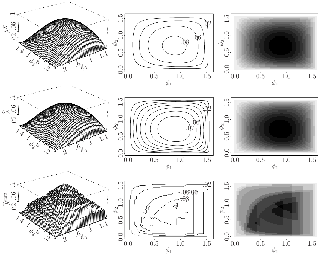
Figure 3.14: From left to right column: perspective, contour and grey-scale image plot of true \lambda^X (\sqrt{3} \cos \phi_1, \sqrt{3} \sin \phi_1 \cos \phi_2, \sqrt{3} \sin \phi_1 \sin \phi_2) with parameters \rho_{12} = 0.3 , \rho_{13} = 0.5 , \rho_{23} = 0.7 and \alpha = 5 (first row) and corresponding estimators based on a particular sample, \hat{\lambda}(\dots; 100, w_1) (middle row) and \hat{\lambda}^{\text{emp}}(\dots; 100) (lower row).
