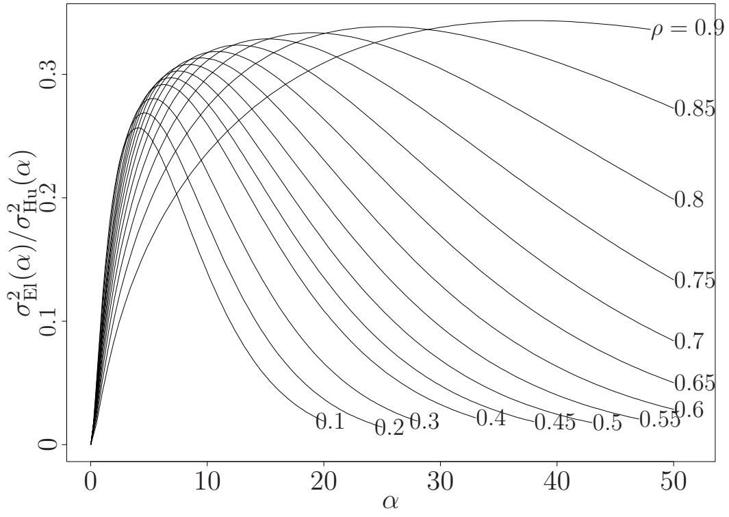
Figure 2.1: Ratio \sigma_{El}^2(\alpha)/\sigma_{Hu}^2(\alpha) for different correlations \rho .
