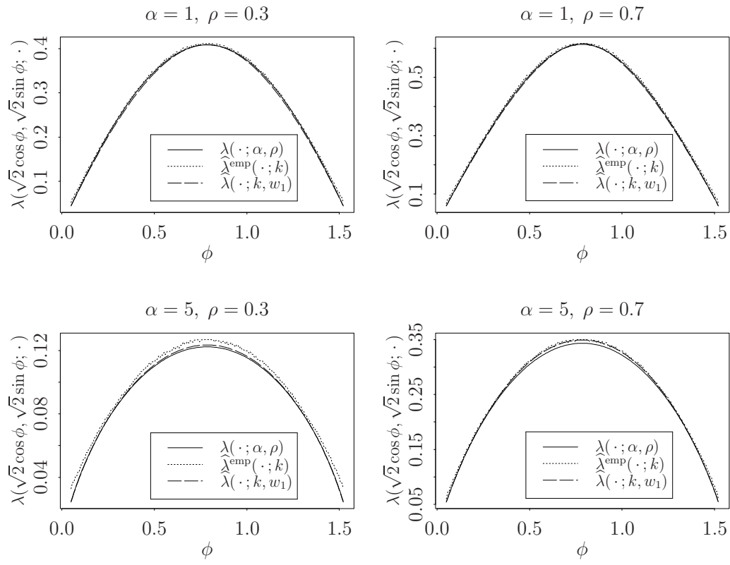
Figure 3.11: Averages of \hat{\lambda}^{\text{emp}}(\sqrt{2}\cos\phi, \sqrt{2}\sin\phi; 50) and \hat{\lambda}(\sqrt{2}\cos\phi, \sqrt{2}\sin\phi; 50, w_1) are plotted against \phi \in (0, \pi/2) .
