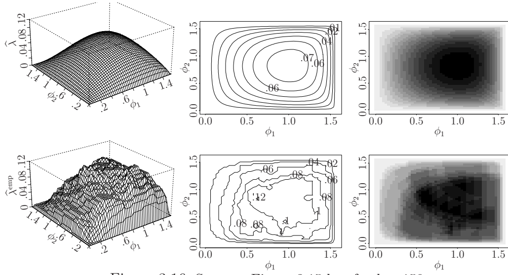
Figure 3.16: Same as Figure 3.15 but for k = 150 .
