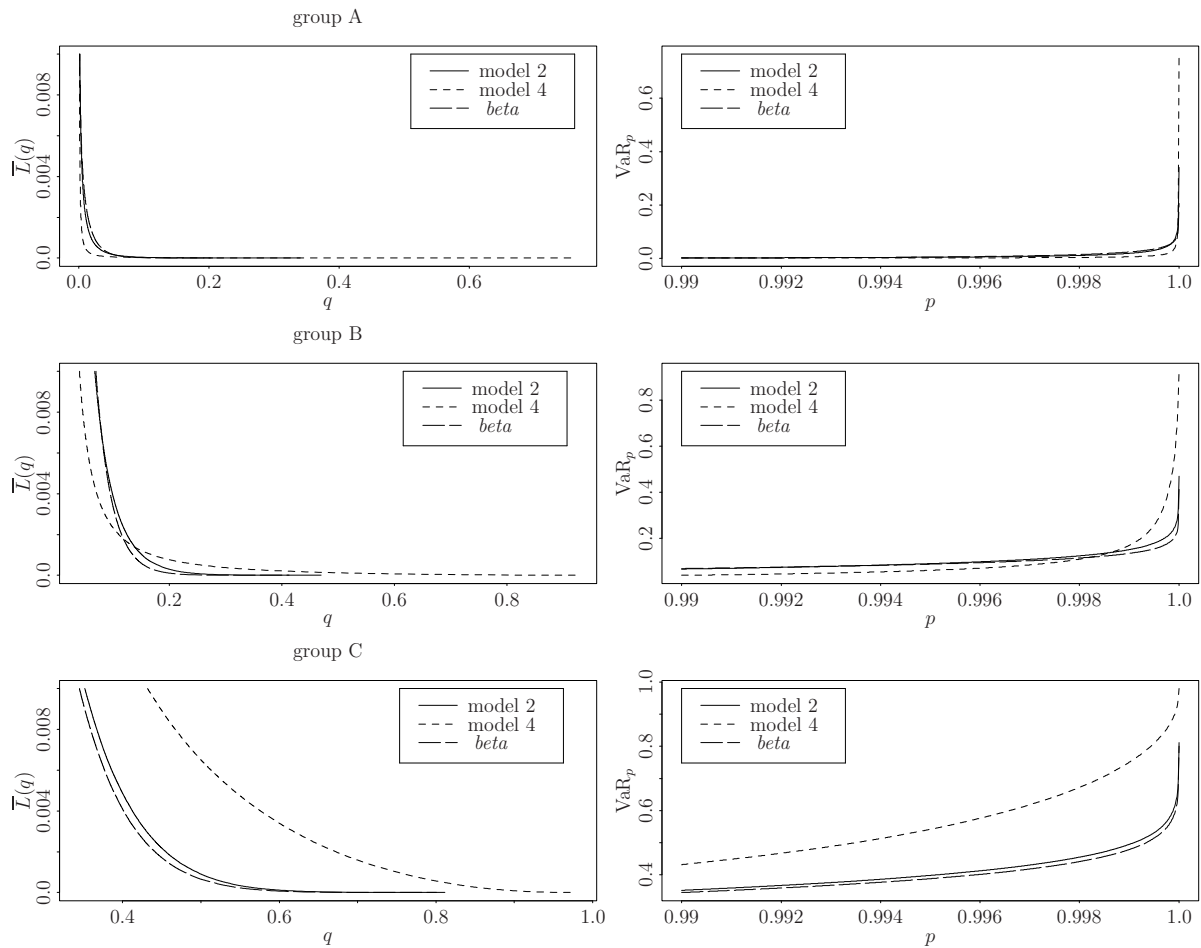
Figure 5.4: Tail-distribution and Value-at-Risk of model 2, 4 and \beta -model in the three groups.
