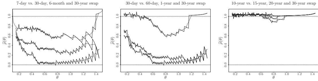
Figure 1.5: Estimates \hat{\rho} for some swap rates with smoothed versions (dashed lines).
