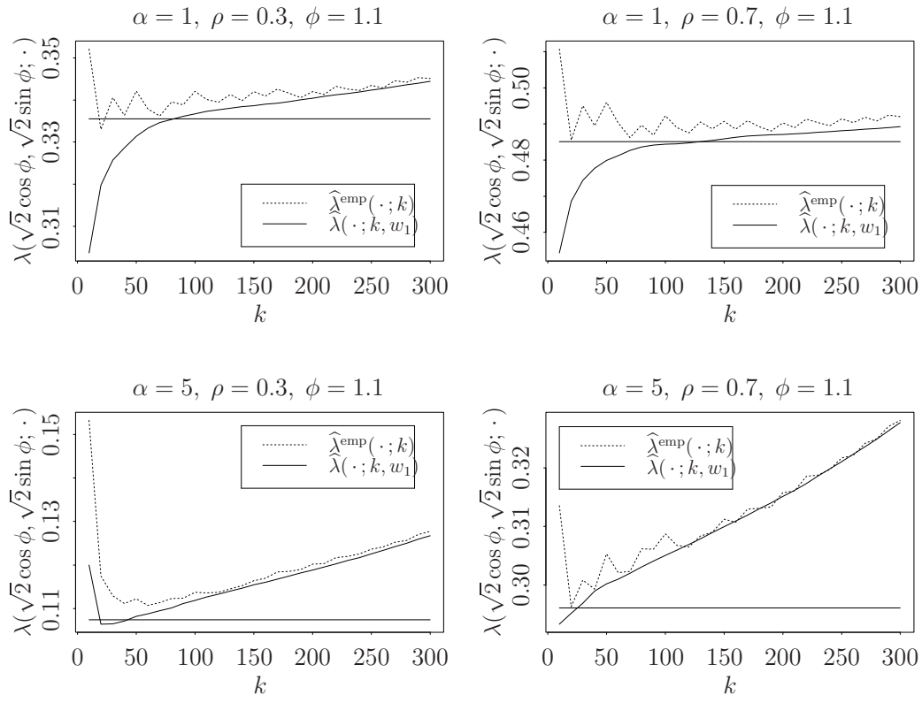
Figure 3.9: Averages of \hat{\lambda}^{\text{emp}}(\sqrt{2} \cos \phi, \sqrt{2} \sin \phi; k) and \hat{\lambda}(\sqrt{2} \cos \phi, \sqrt{2} \sin \phi; k, w_1) with \phi = 1.1 are plotted against k = 10, 20, \dots, 300 .
