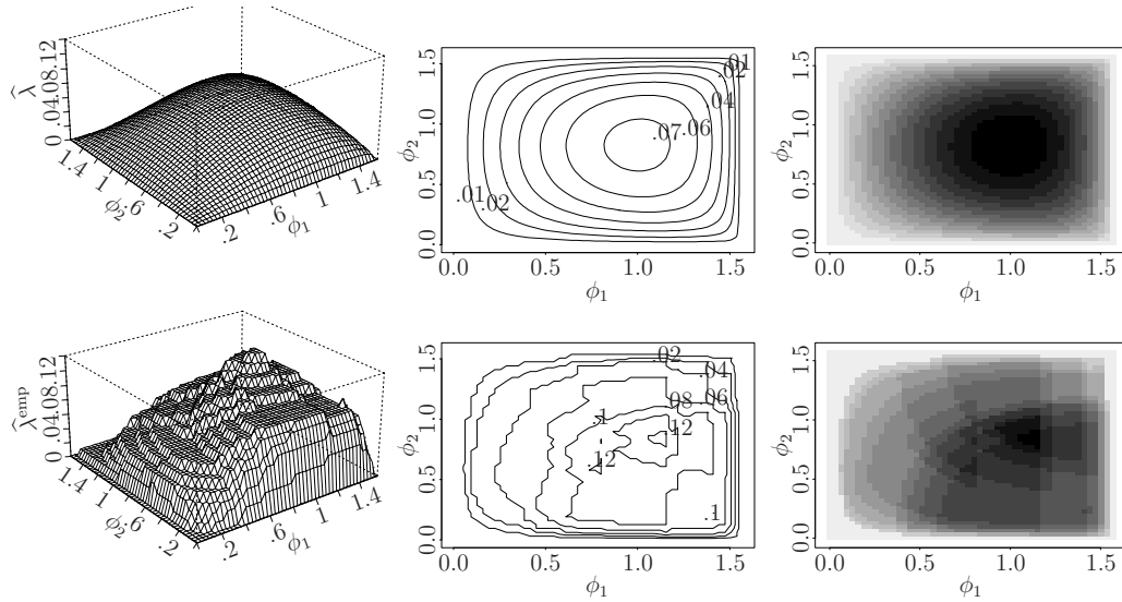
Figure 3.15: From left to right column: perspective, contour and grey-scale image plot of estimators \hat{\lambda}(\dots; 100, w_1) (upper row) and \hat{\lambda}^{\text{emp}}(\dots; 100) (lower row) of currencies (GBP, USD, CHF).
