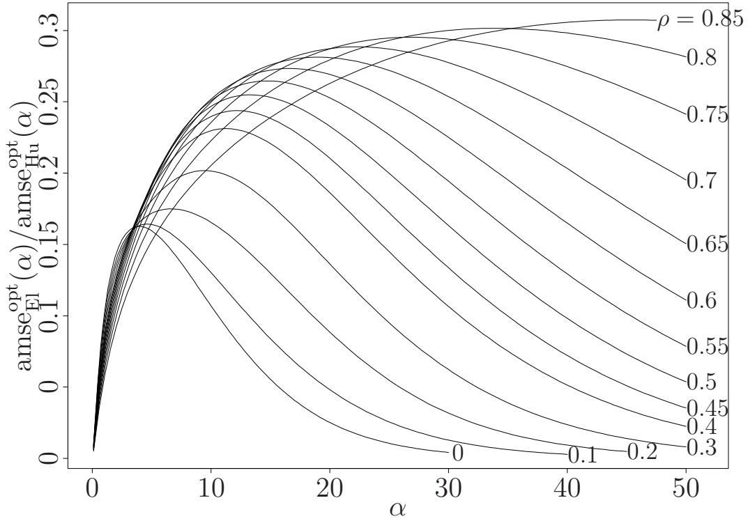
Figure 2.2: Ratio \text{amse}_{El}^{\text{opt}}(\alpha)/\text{amse}_{Hu}^{\text{opt}}(\alpha) for different correlations \rho and \beta = -\alpha .
