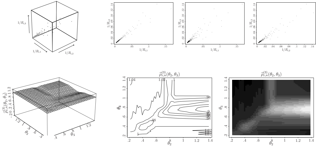
Figure 1.8: First row: data (3-d and 2-d projections) of the ranks 1/R_{i,j} , 1 \leq j \leq 3 , of the high dependent 5-year, 6-year and 7-year EUR swap rates.
