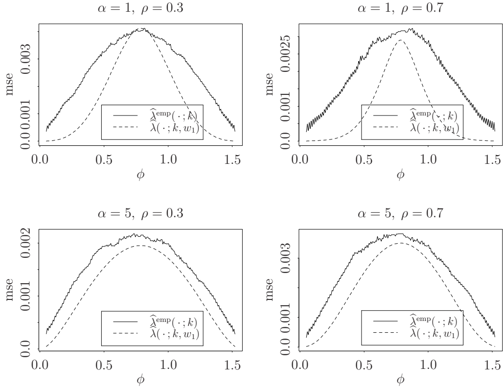
Figure 3.12: Estimated mean squared errors of estimators in Figure 3.11.
