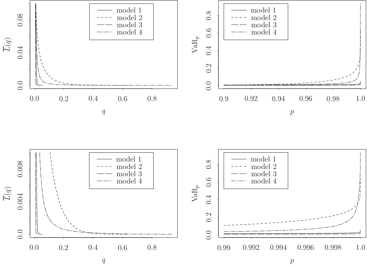
Figure 5.2: Tail-distribution and Value-at-Risk of the four models with group B -parameter setting.
