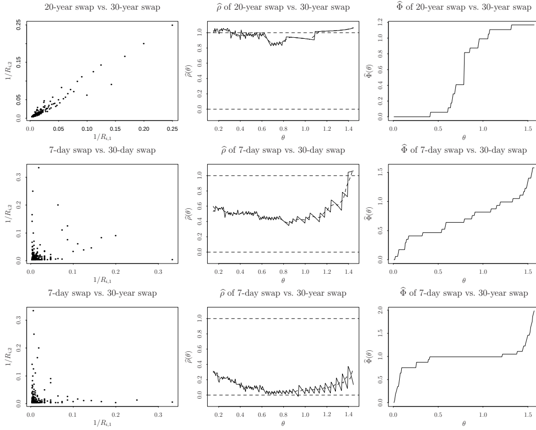
Figure 1.6: Estimators of \rho and \Phi for some swap rates: 20-year vs. 30-year (first row), 7-day vs. 30-day (second row), and 7-day vs. 30-year swap rates (third row).
