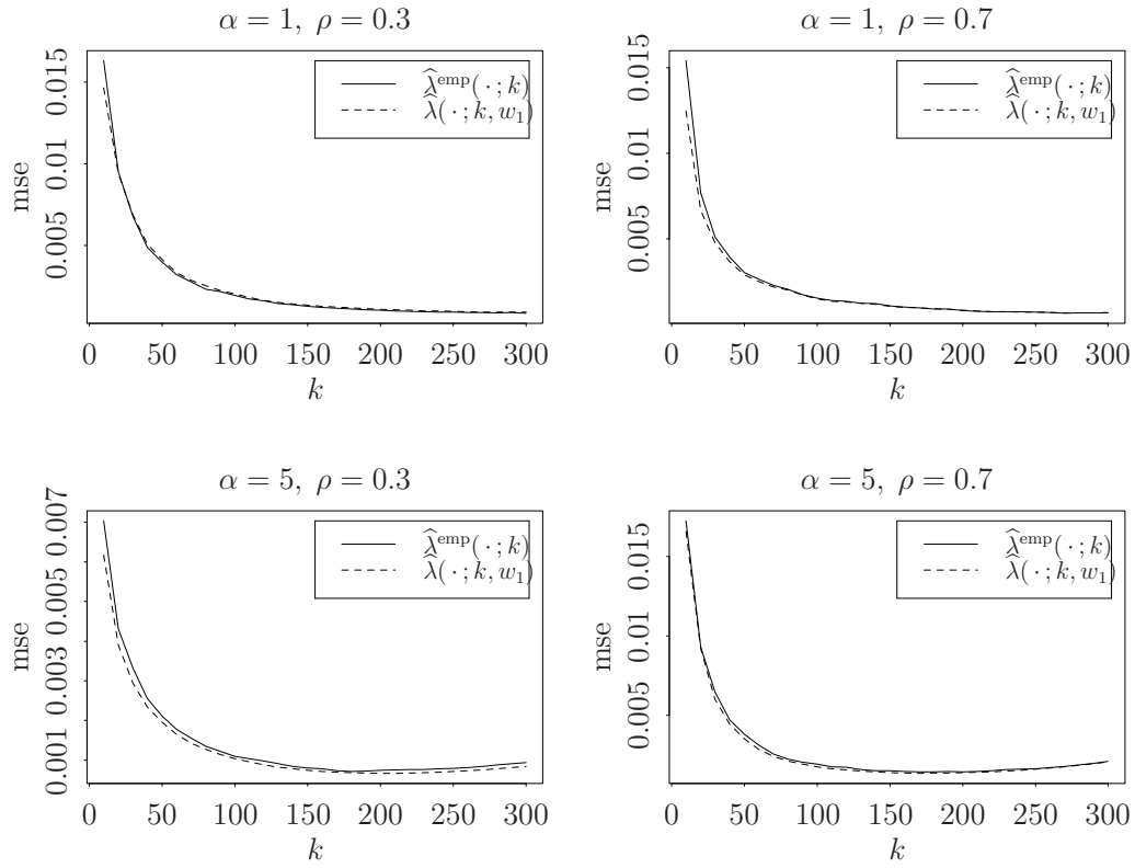
Figure 3.6: Estimated mean squared errors of estimators in Figure 3.5.
