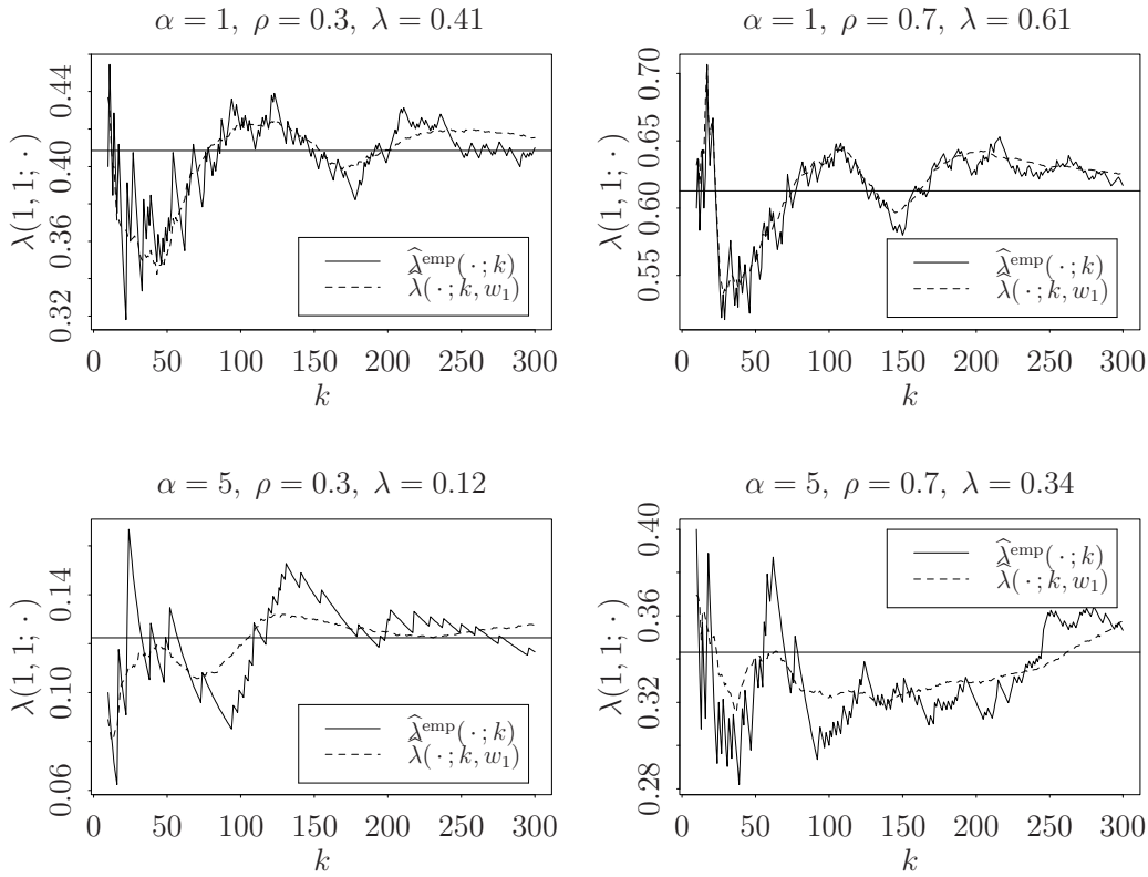
Figure 3.8: Estimators \hat{\lambda}^{\text{emp}}(1, 1, k) and \hat{\lambda}(1, 1, k, w_1) based on a particular sample are plotted against k = 10, 11, \dots, 300 .
