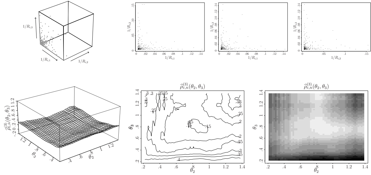
Figure 1.7: First row: data (3-d and 2-d projections) of the ranks 1/R_{i,j} , 1 \leq j \leq 3 , of the low dependent 7-day swap rates rates in USD, EUR and GBP.
