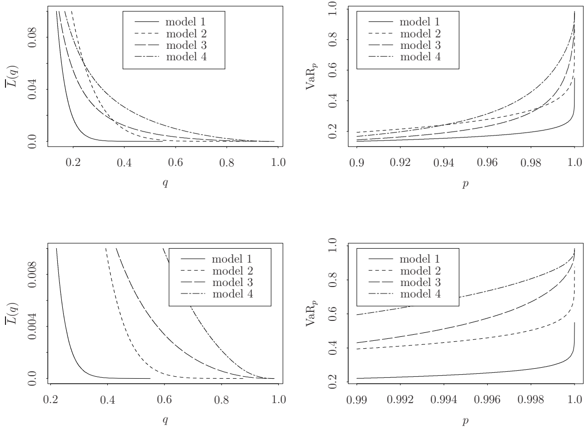
Figure 5.3: Tail-distribution and Value-at-Risk of the four models with group C -parameter setting.
