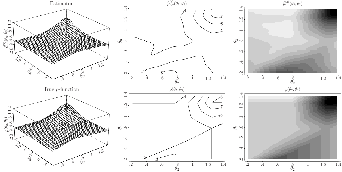
Figure 1.4: First row: smoothed estimate \hat{\rho}_{\varepsilon,n}^{(3)}(\theta_2, \theta_3) of the simulated data (see Figure 1.3), with perspective plot (left-most), contour plot (middle) and image plot (right-most).
