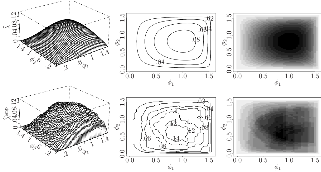
Figure 3.17: Same as Figure 3.15 but for k = 200 .
