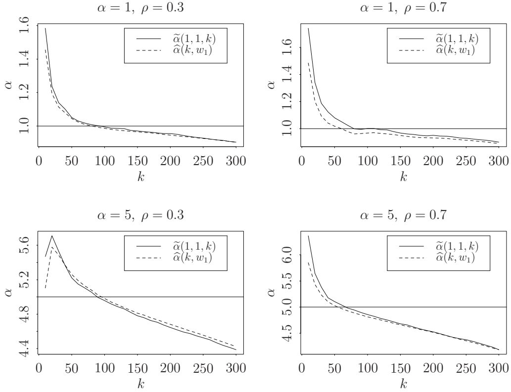
Figure 3.3: Averages of \tilde{\alpha}(1, 1, k) and \hat{\alpha}(k, w_1) are plotted against k = 10, 20, \dots, 300 .
