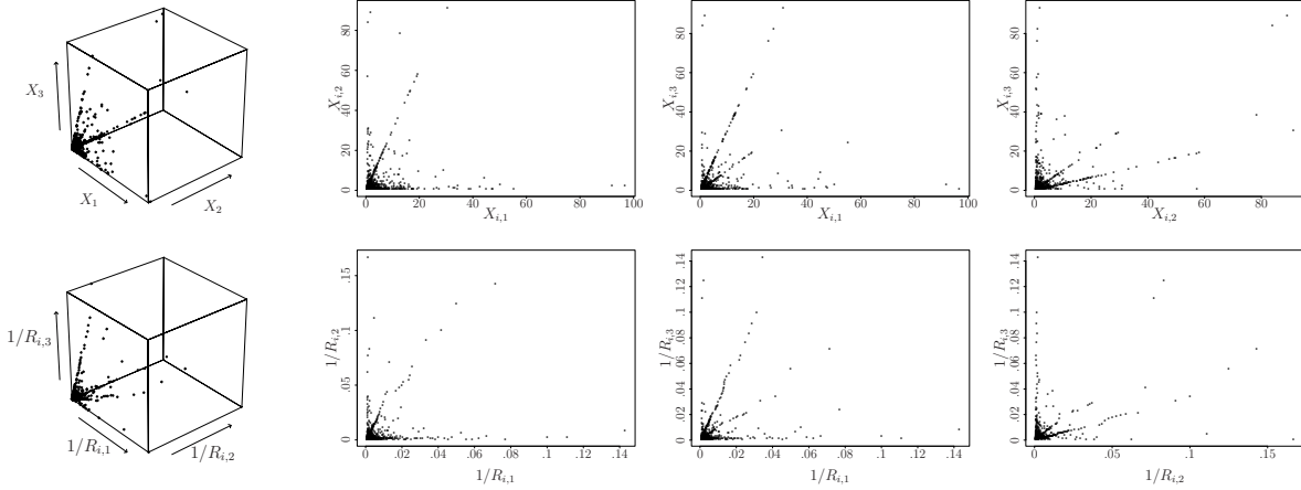
Figure 1.3: First row: data (3-d and 2-d projections) of the model given in Example 1.5.2.
