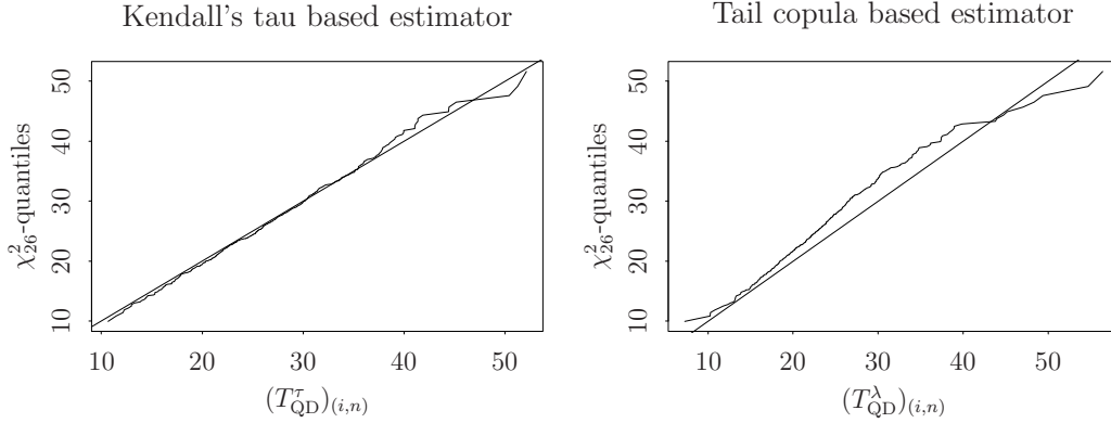
Figure 4.1: QQ -plot of ordered estimates \hat{T} against the \chi^2_{26} -quantiles.
