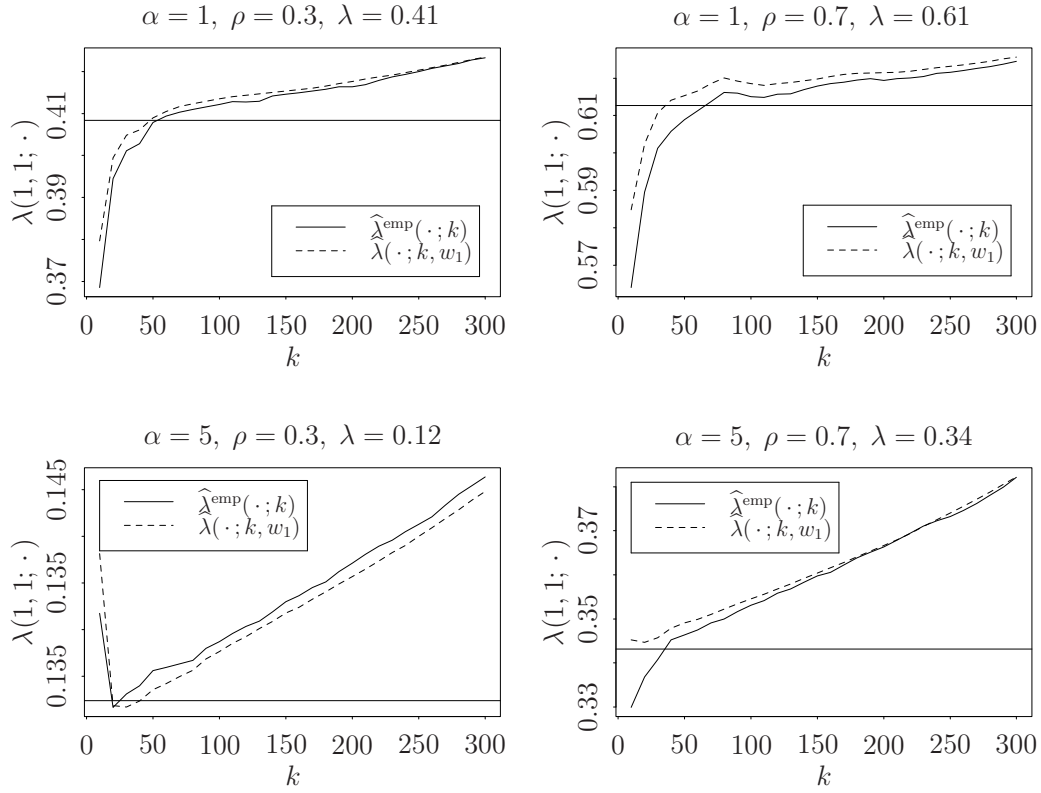
Figure 3.5: Averages of \hat{\lambda}^{\text{emp}}(1, 1; k) and \hat{\lambda}(1, 1; k, w_1) are plotted against k = 10, 20, \dots, 300 .
