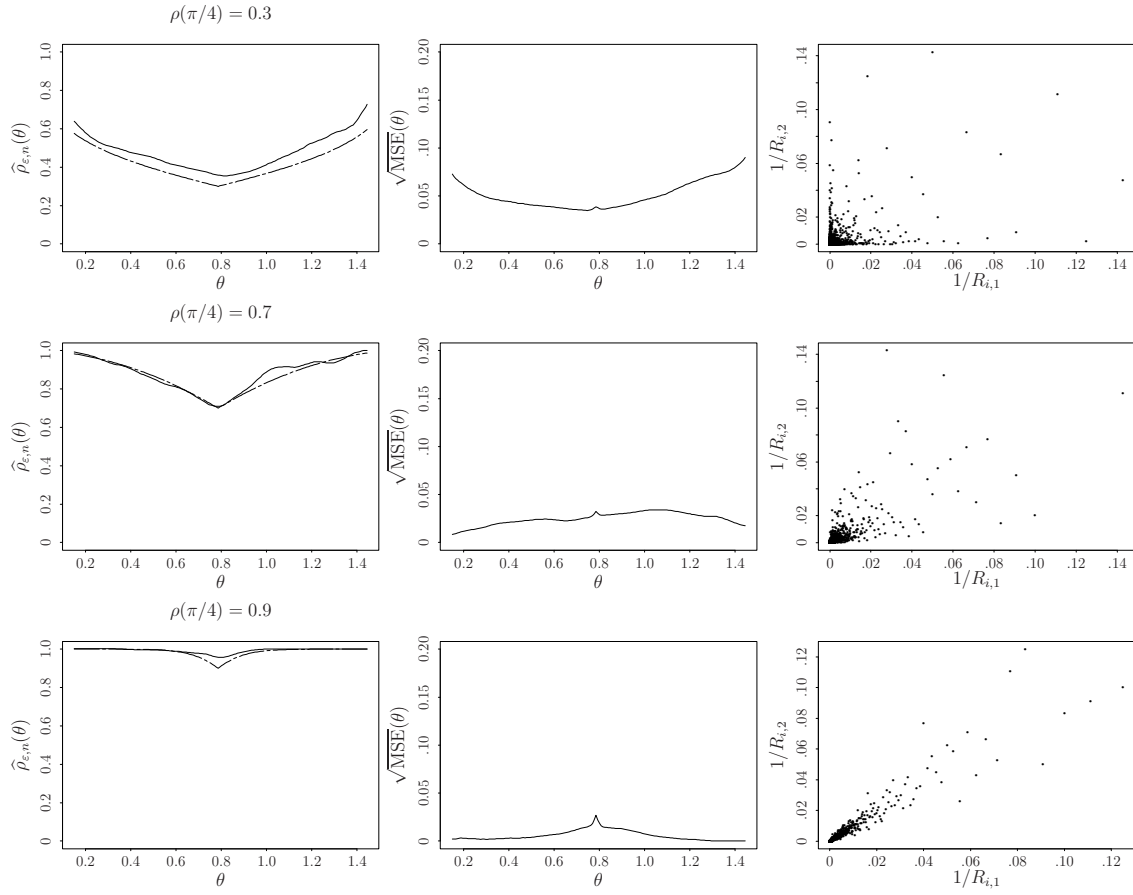
Figure 1.2: Left column: smoothed versions \hat{\rho}_{\varepsilon,n}^{(5)}(\theta) (solid line) overlaid with true function \rho(\theta) . Middle column: \sqrt{\text{MSE}}(\theta) . Right column: plots of 1/R_{i,j} , j = 1, 2 , for C_{\mathbf{X}} given in (1.4.3) and \rho(\pi/4) = 0.3 (upper row), \rho(\pi/4) = 0.7 (middle row), \rho(\pi/4) = 0.9 (lower row).
