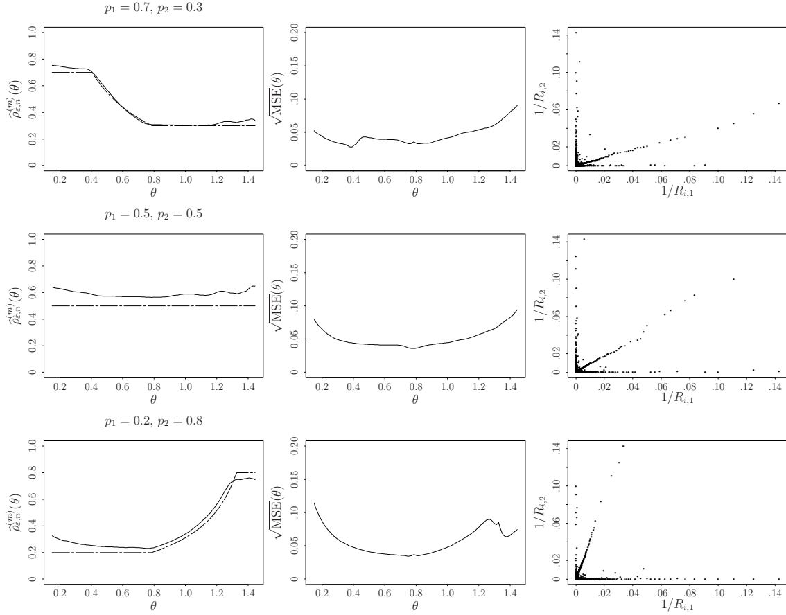
Figure 1.1: Left column: smoothed version of \hat{\rho}_{\varepsilon,n}^{(5)}(\theta) (solid line) overlaid with true function \rho(\theta) . Middle column: \sqrt{\text{MSE}}(\theta) . Right column: plots of (1/R_{i,1}, 1/R_{i,2}) , with points close to (1,1) truncated, p_1 = 0.7, p_2 = 0.3 (upper row), p_1 = 0.5, p_2 = 0.5 (middle row) and p_1 = 0.2, p_2 = 0.8 (lower row).
