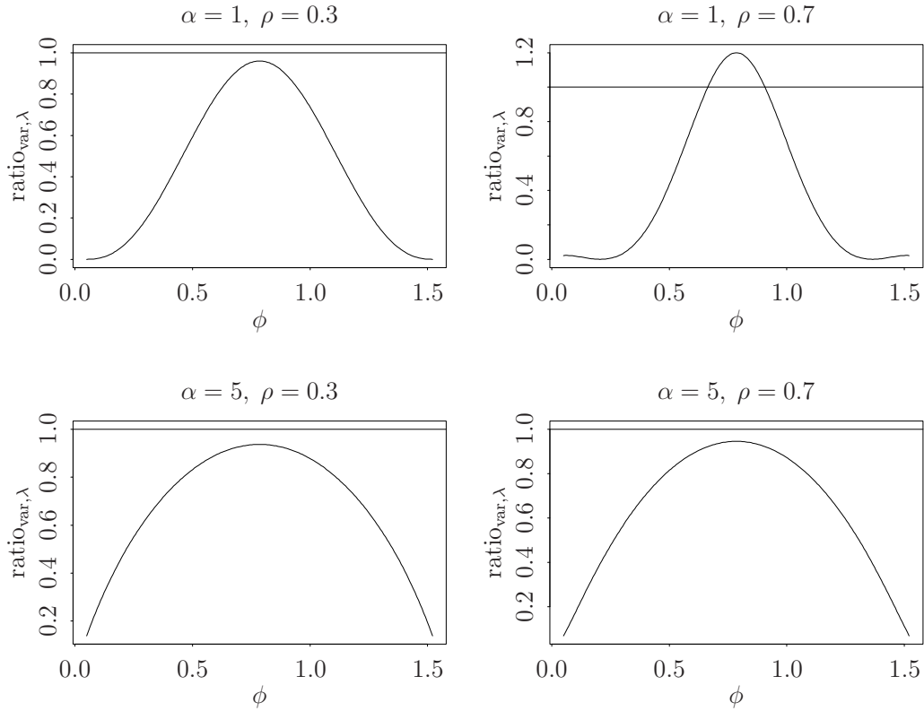
Figure 3.2: Theoretical ratios, \text{ratio}_{\text{var}, \lambda} , are plotted against \phi \in (0, \pi/2) for (\alpha, \rho) \in \{1, 5\} \times \{0.3, 0.7\} .
