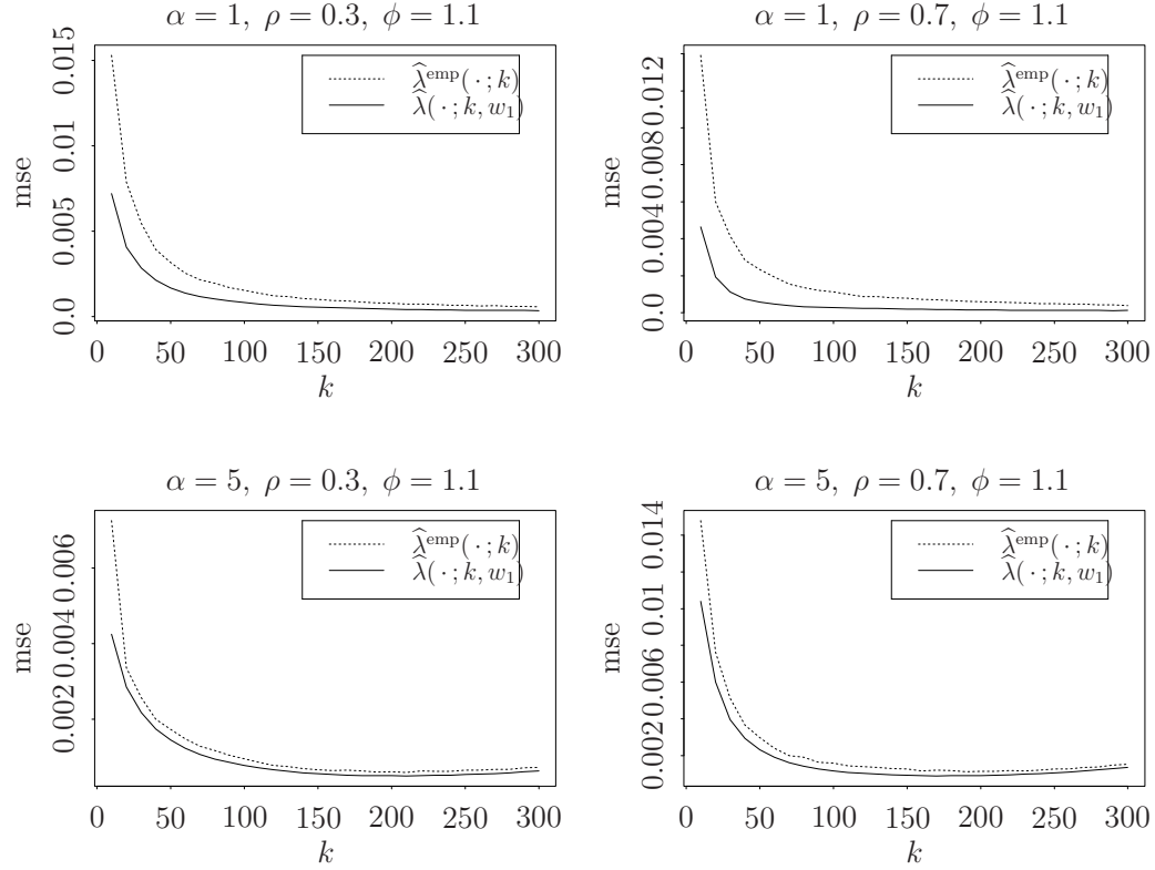
Figure 3.10: Estimated mean squared errors of estimators in Figure 3.9.
