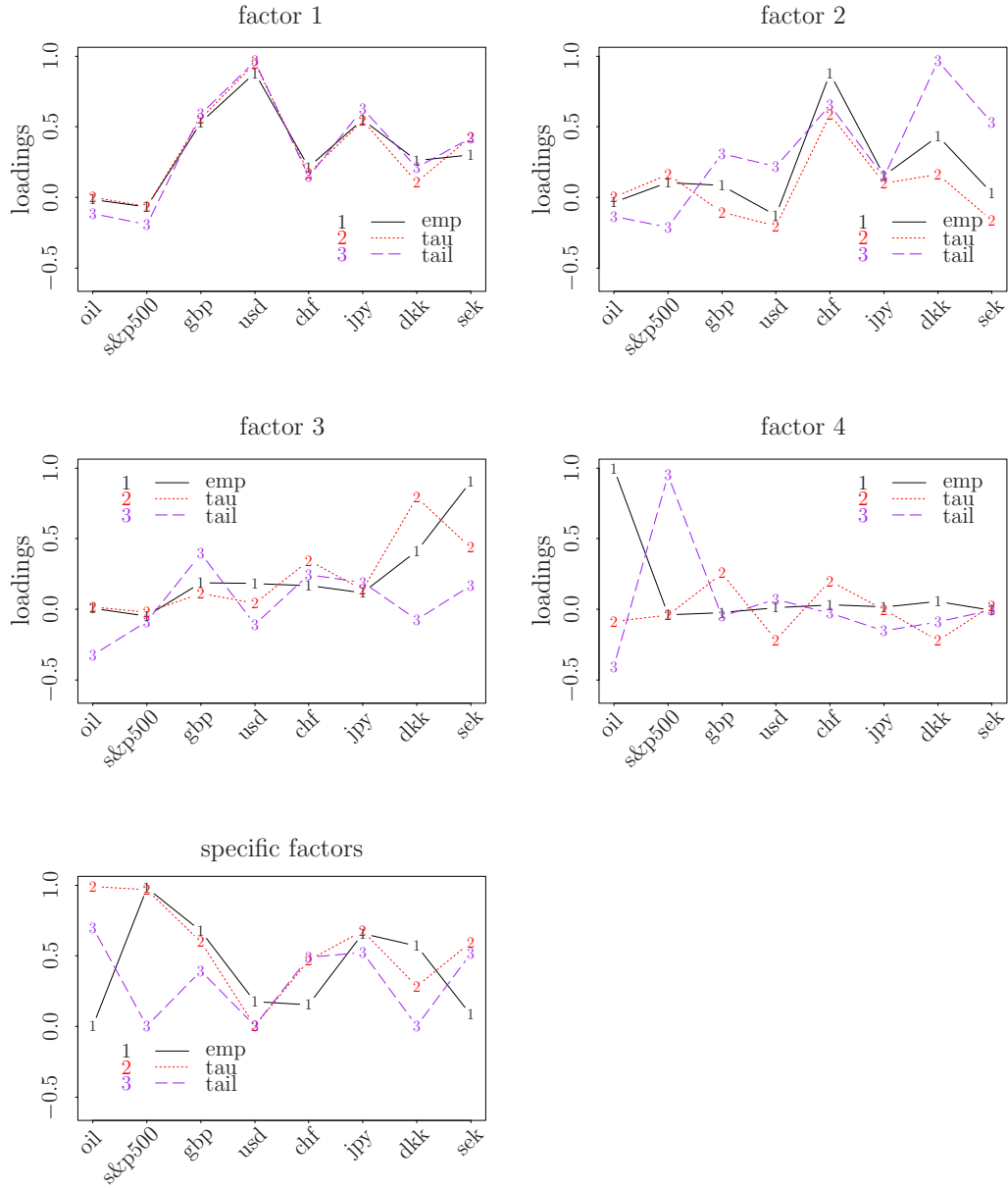
Figure 4.2: Oil-currency data: factor analysis based on 4 factors and different statistics, "emp" for the loadings \hat{\boldsymbol{\vartheta}}_{\text{emp}} , "tau" for \hat{\boldsymbol{\vartheta}}_{\tau} and "tail" for \hat{\boldsymbol{\vartheta}}_{\lambda} .
