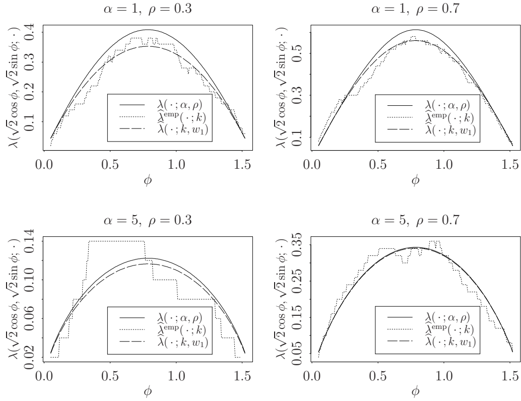
Figure 3.13: Estimators \hat{\lambda}^{\text{emp}}(\sqrt{2} \cos \phi, \sqrt{2} \sin \phi; 50) and \hat{\lambda}(\sqrt{2} \cos \phi, \sqrt{2} \sin \phi; 50, w_1) based on a particular sample are plotted against \phi \in (0, \pi/2) .
