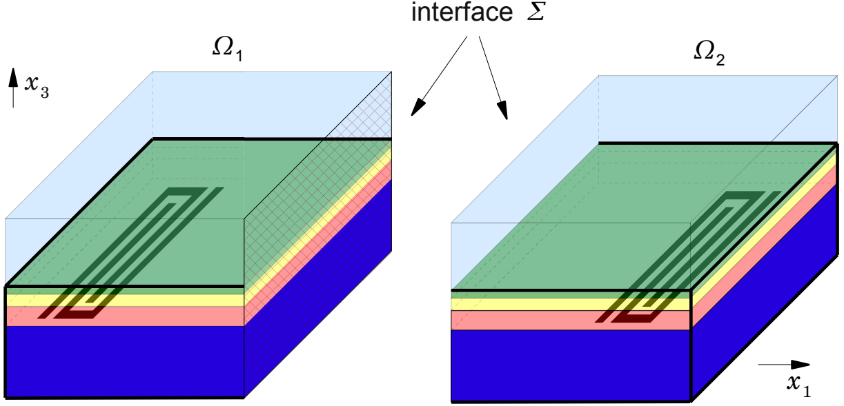
Figure 2.4: Domain decomposition.
