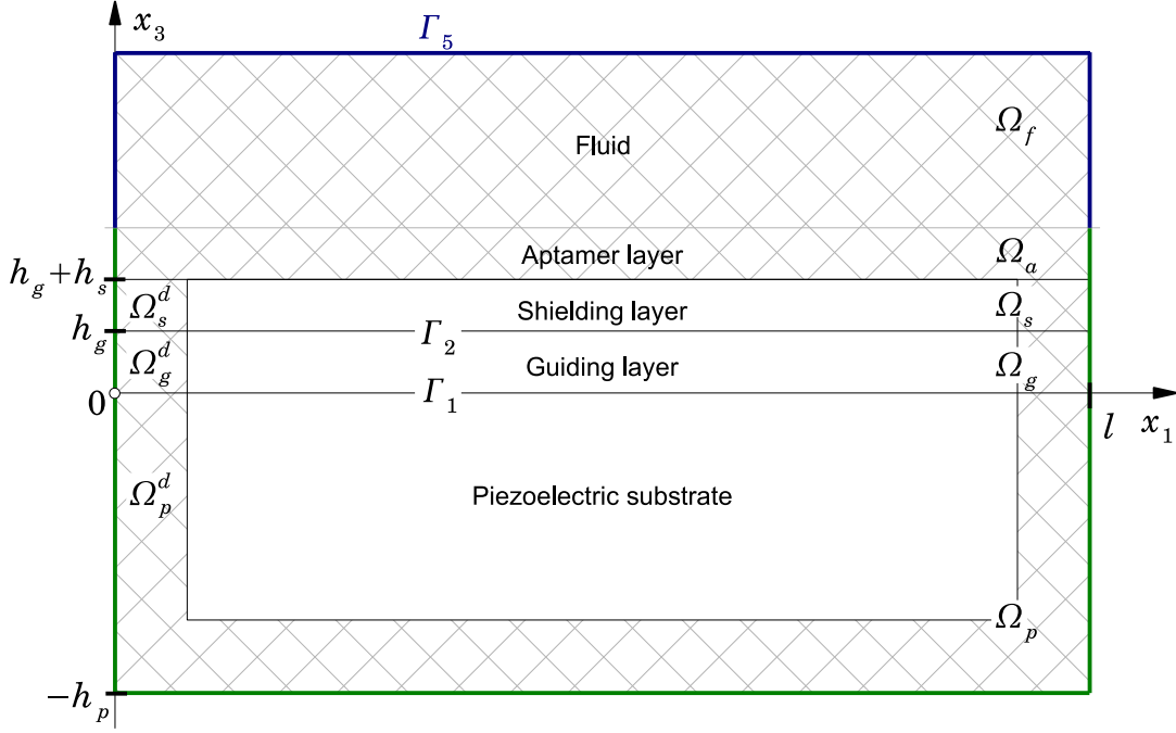
Figure 2.3: Cross section of the domain. The subdomain where \mathbf{v} = 0 is hatched.
